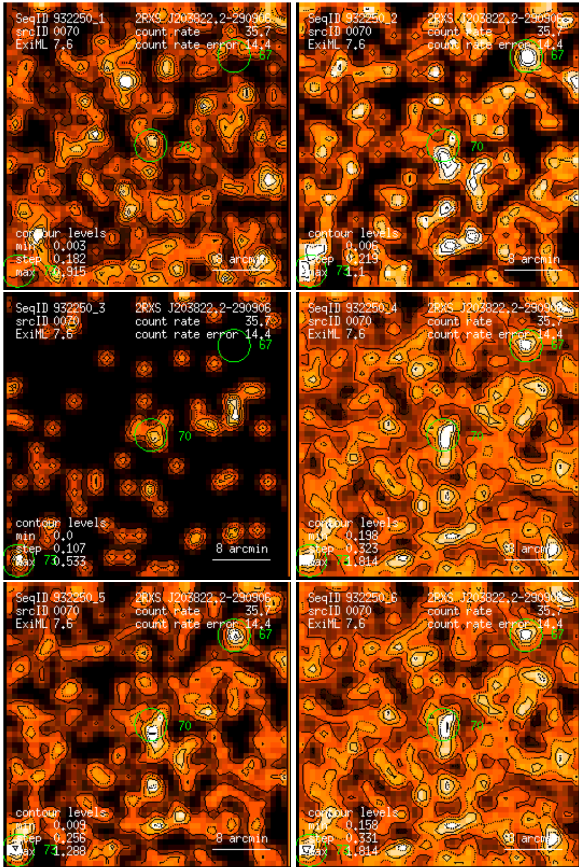
Figure 70: RASS 932250: detection 0070: band rate images, Gaussian filter: (1) PSPC channels 11 – 41, (2) 52 – 90, (3) 91 – 201, (4) 11 – 235, (5) 52 – 201, (6) 11 – 201. Broad band rates in counts/ks. Band rate contour levels in counts/ks/arcmin 2 .
