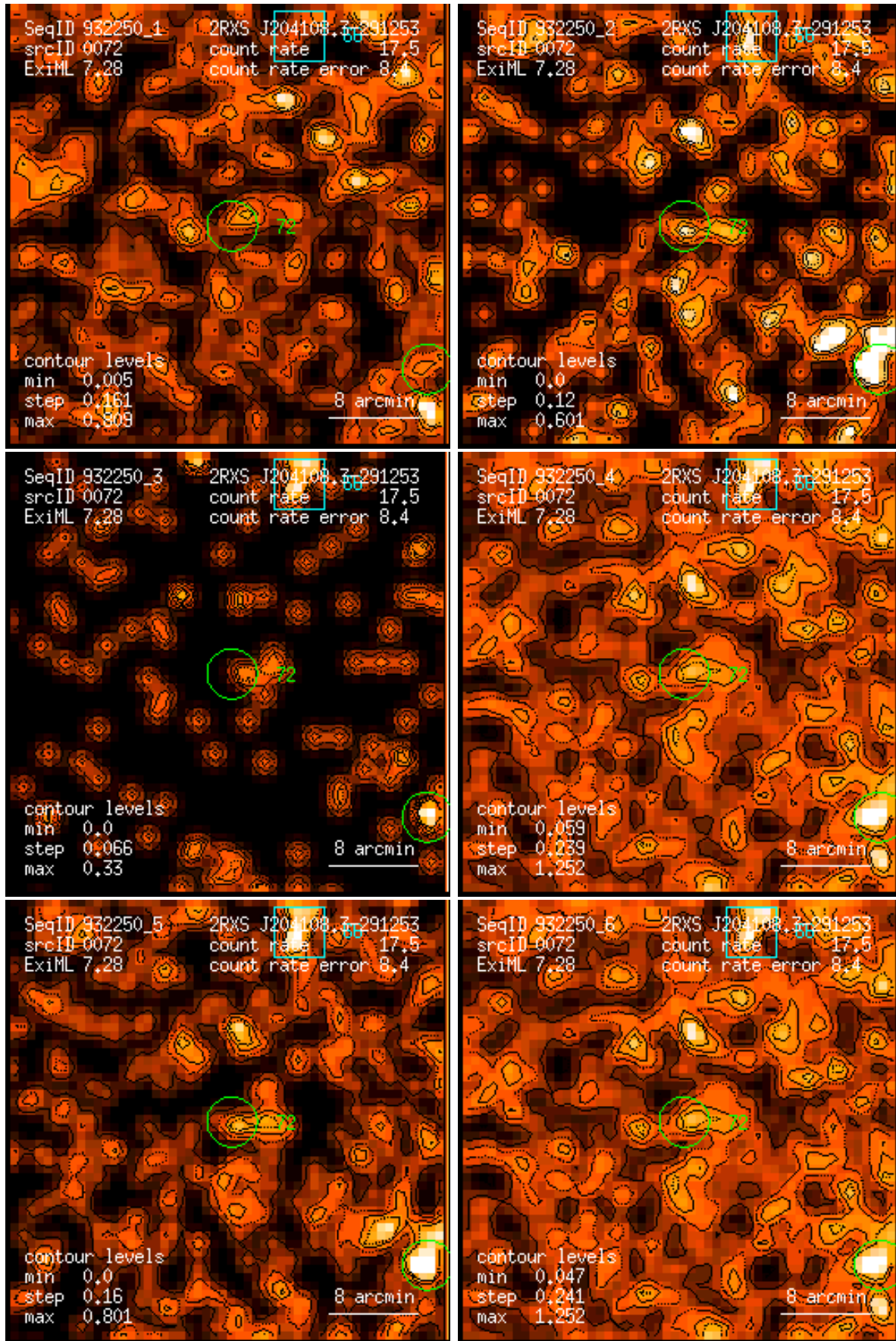
Figure 72: RASS 932250: detection 0072: band rate images, Gaussian filter: (1) PSPC channels 11 – 41, (2) 52 – 90, (3) 91 – 201, (4) 11 – 235, (5) 52 – 201, (6) 11 – 201. Broad band rates in counts/ks. Band rate contour levels in counts/ks/arcmin 2 .
