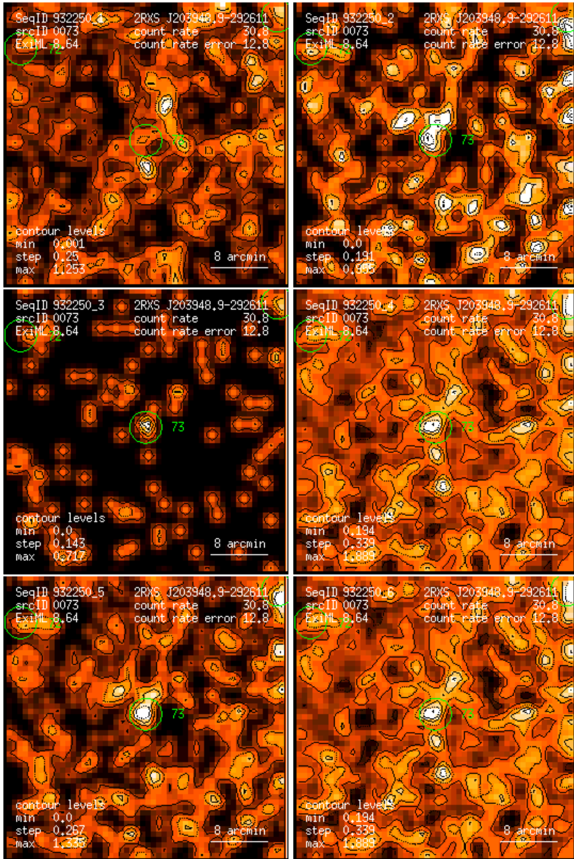
Figure 73: RASS 932250: detection 0073: band rate images, Gaussian filter: (1) PSPC channels 11 – 41, (2) 52 – 90, (3) 91 – 201, (4) 11 – 235, (5) 52 – 201, (6) 11 – 201. Broad band rates in counts/ks. Band rate contour levels in counts/ks/arcmin 2 .
