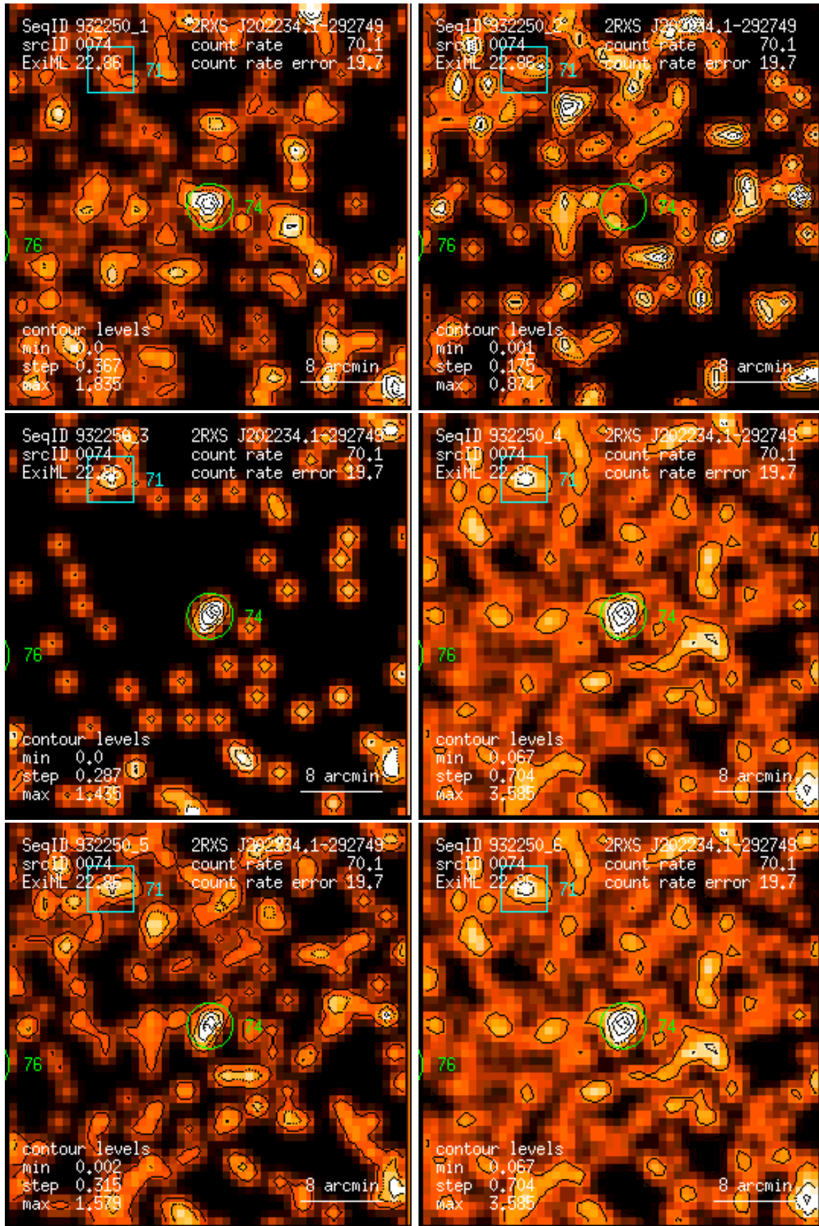
Figure 74: RASS 932250: detection 0074: band rate images, Gaussian filter: (1) PSPC channels 11 – 41, (2) 52 – 90, (3) 91 – 201, (4) 11 – 235, (5) 52 – 201, (6) 11 – 201. Broad band rates in counts/ks. Band rate contour levels in counts/ks/arcmin 2 .
