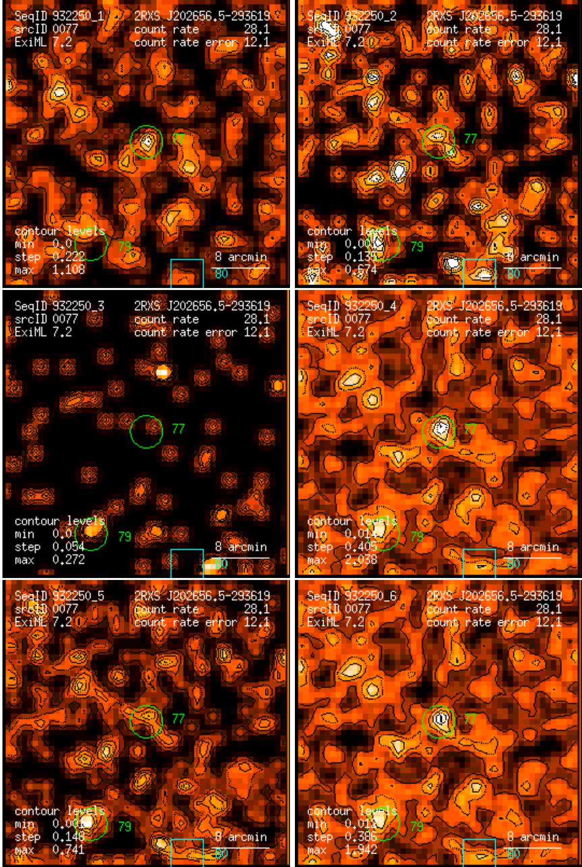
Figure 77: RASS 932250: detection 0077: band rate images, Gaussian filter: (1) PSPC channels 11 – 41, (2) 52 – 90, (3) 91 – 201, (4) 11 – 235, (5) 52 – 201, (6) 11 – 201. Broad band rates in counts/ks. Band rate contour levels in counts/ks/arcmin 2 .
