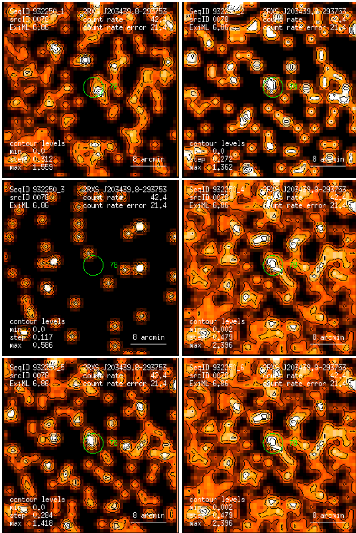
Figure 78: RASS 932250: detection 0078: band rate images, Gaussian filter: (1) PSPC channels 11 – 41, (2) 52 – 90, (3) 91 – 201, (4) 11 – 235, (5) 52 – 201, (6) 11 – 201. Broad band rates in counts/ks. Band rate contour levels in counts/ks/arcmin 2 .
