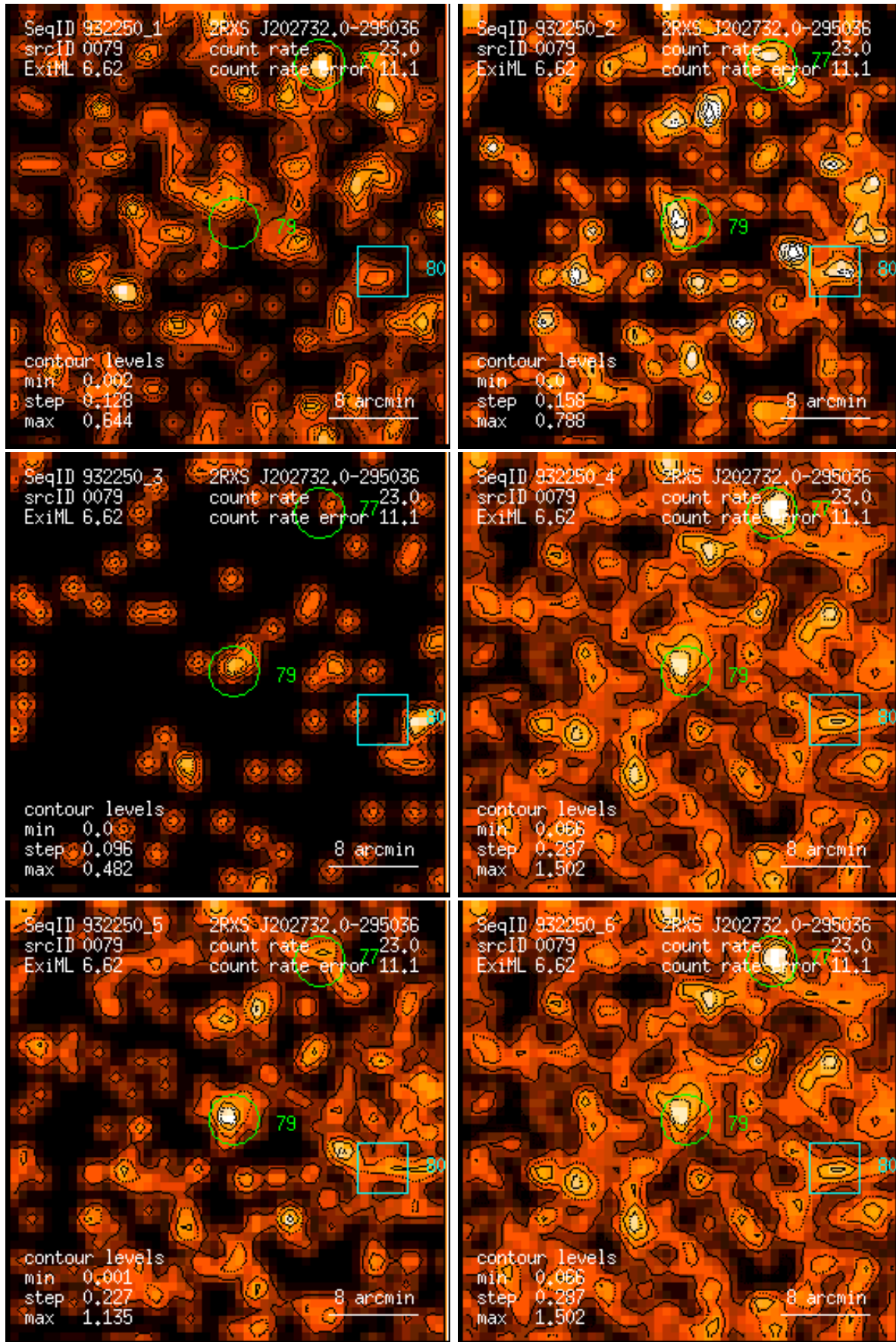
Figure 79: RASS 932250: detection 0079: band rate images, Gaussian filter: (1) PSPC channels 11 – 41, (2) 52 – 90, (3) 91 – 201, (4) 11 – 235, (5) 52 – 201, (6) 11 – 201. Broad band rates in counts/ks. Band rate contour levels in counts/ks/arcmin 2 .
