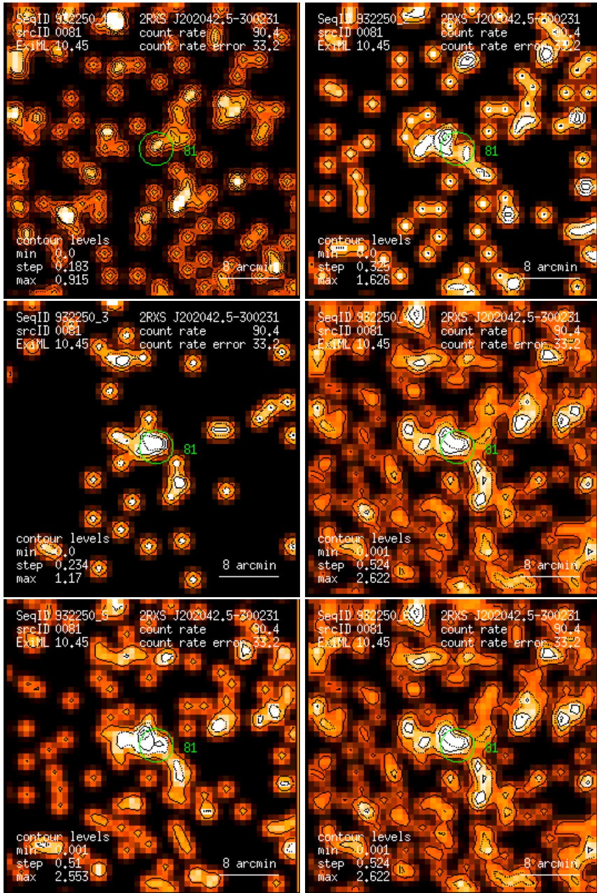
Figure 81: RASS 932250: detection 0081: band rate images, Gaussian filter: (1) PSPC channels 11 – 41, (2) 52 – 90, (3) 91 – 201, (4) 11 – 235, (5) 52 – 201, (6) 11 – 201. Broad band rates in counts/ks. Band rate contour levels in counts/ks/arcmin 2 .
