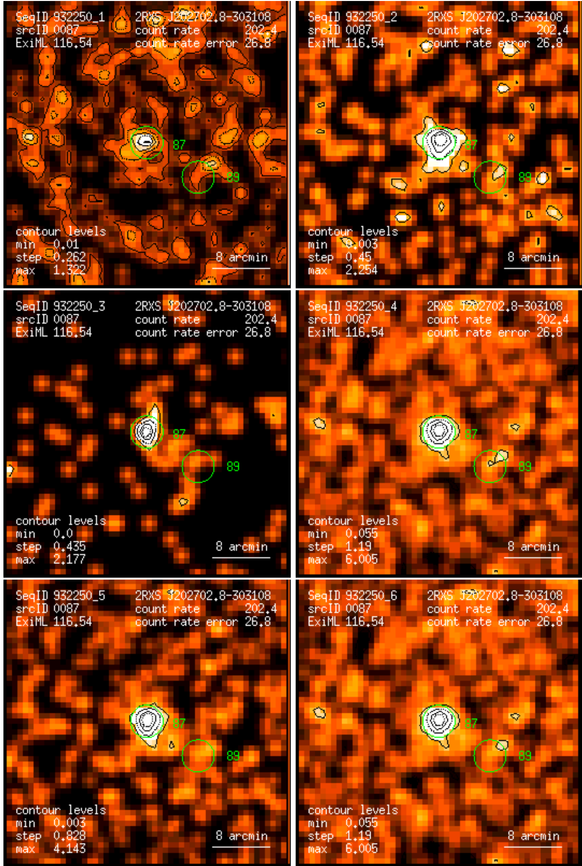
Figure 87: RASS 932250: detection 0087: band rate images, Gaussian filter: (1) PSPC channels 11 – 41, (2) 52 – 90, (3) 91 – 201, (4) 11 – 235, (5) 52 – 201, (6) 11 – 201. Broad band rates in counts/ks. Band rate contour levels in counts/ks/arcmin 2 .
