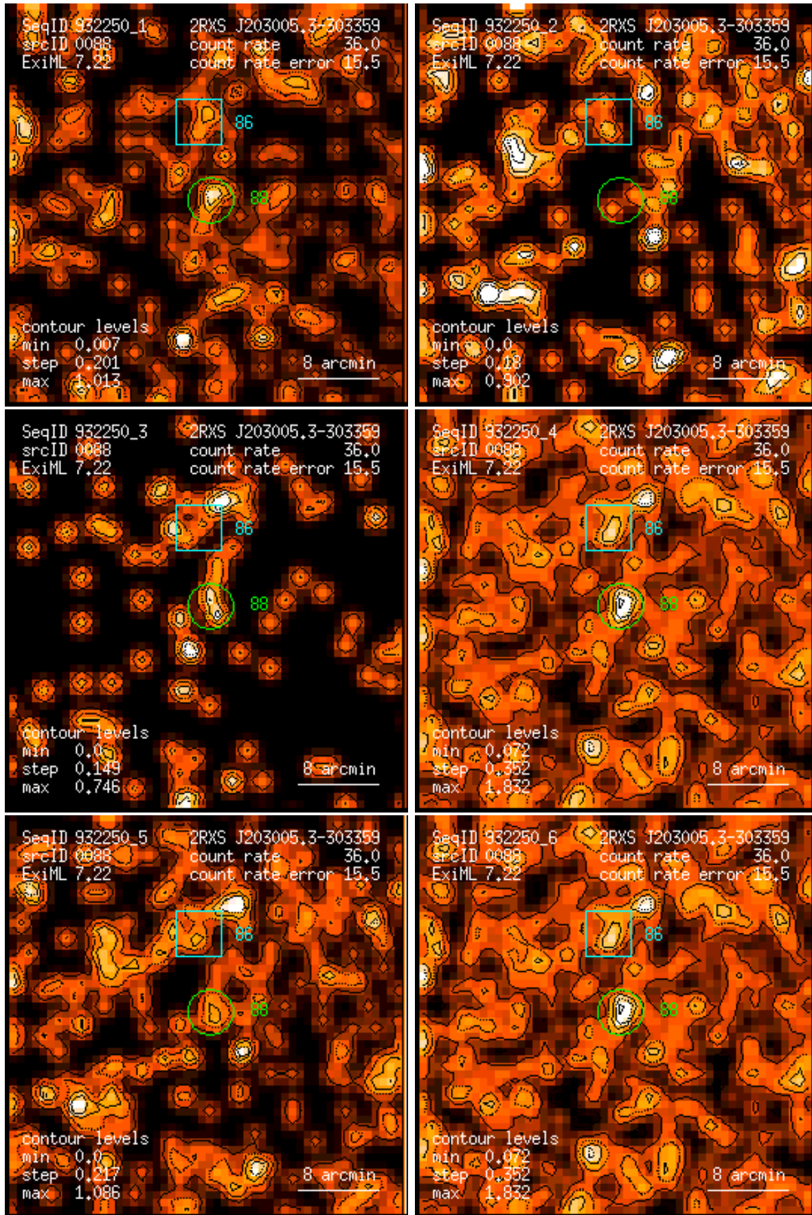
Figure 88: RASS 932250: detection 0088: band rate images, Gaussian filter: (1) PSPC channels 11 – 41, (2) 52 – 90, (3) 91 – 201, (4) 11 – 235, (5) 52 – 201, (6) 11 – 201. Broad band rates in counts/ks. Band rate contour levels in counts/ks/arcmin 2 .
