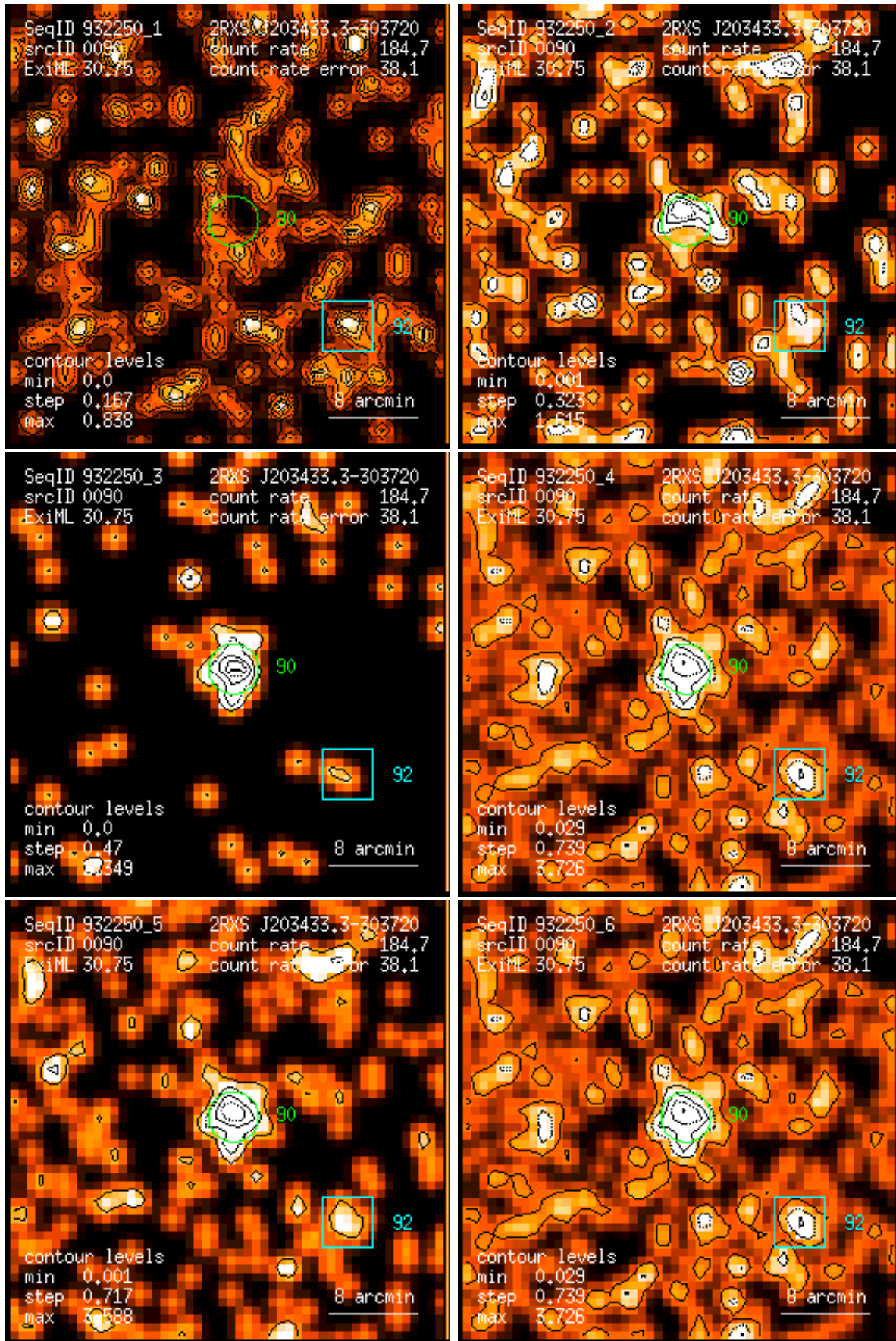
Figure 90: RASS 932250: detection 0090: band rate images, Gaussian filter: (1) PSPC channels 11 – 41, (2) 52 – 90, (3) 91 – 201, (4) 11 – 235, (5) 52 – 201, (6) 11 – 201. Broad band rates in counts/ks. Band rate contour levels in counts/ks/arcmin 2 .
