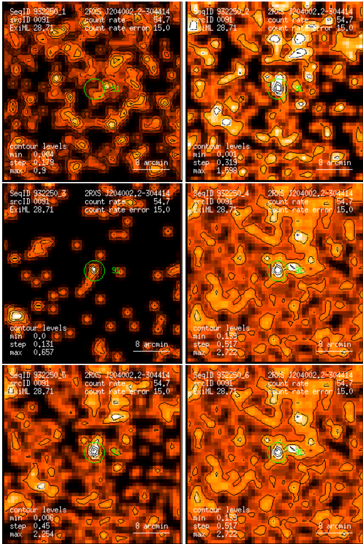
Figure 91: RASS 932250: detection 0091: band rate images, Gaussian filter: (1) PSPC channels 11 – 41, (2) 52 – 90, (3) 91 – 201, (4) 11 – 235, (5) 52 – 201, (6) 11 – 201. Broad band rates in counts/ks. Band rate contour levels in counts/ks/arcmin 2 .
