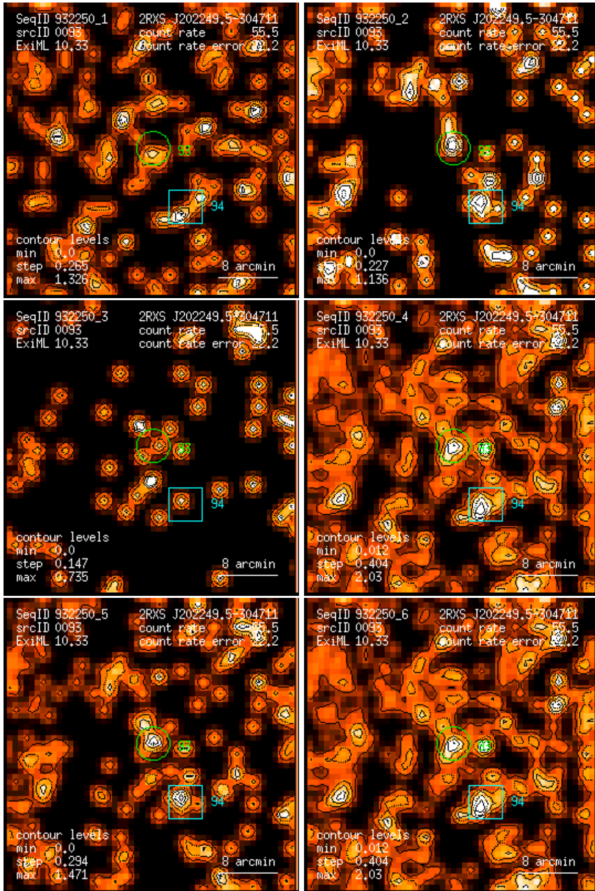
Figure 93: RASS 932250: detection 0093: band rate images, Gaussian filter: (1) PSPC channels 11 – 41, (2) 52 – 90, (3) 91 – 201, (4) 11 – 235, (5) 52 – 201, (6) 11 – 201. Broad band rates in counts/ks. Band rate contour levels in counts/ks/arcmin 2 .
