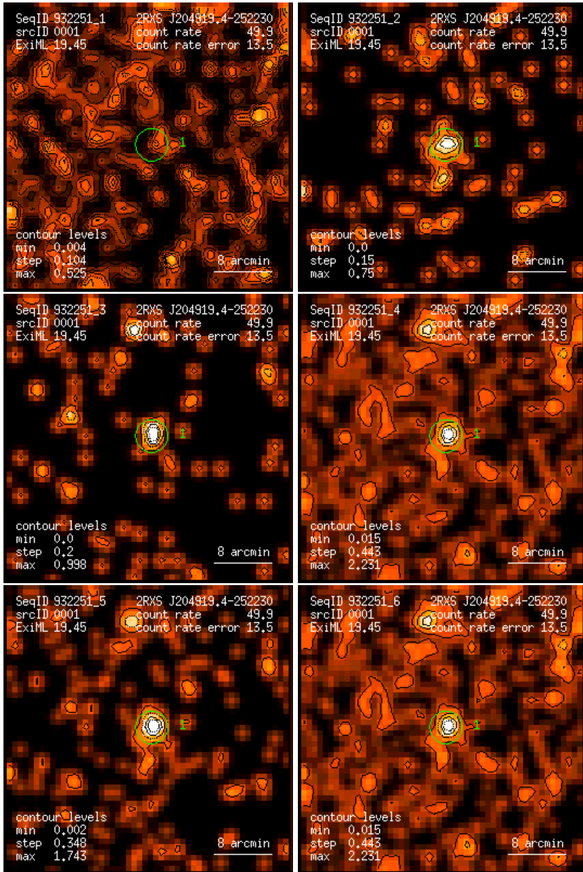
Figure 1: RASS 932251: detection 0001: band rate images, Gaussian filter: (1) PSPC channels 11 – 41, (2) 52 – 90, (3) 91 – 201, (4) 11 – 235, (5) 52 – 201, (6) 11 – 201. Broad band rates in counts/ks. Band rate contour levels in counts/ks/arcmin 2 .
