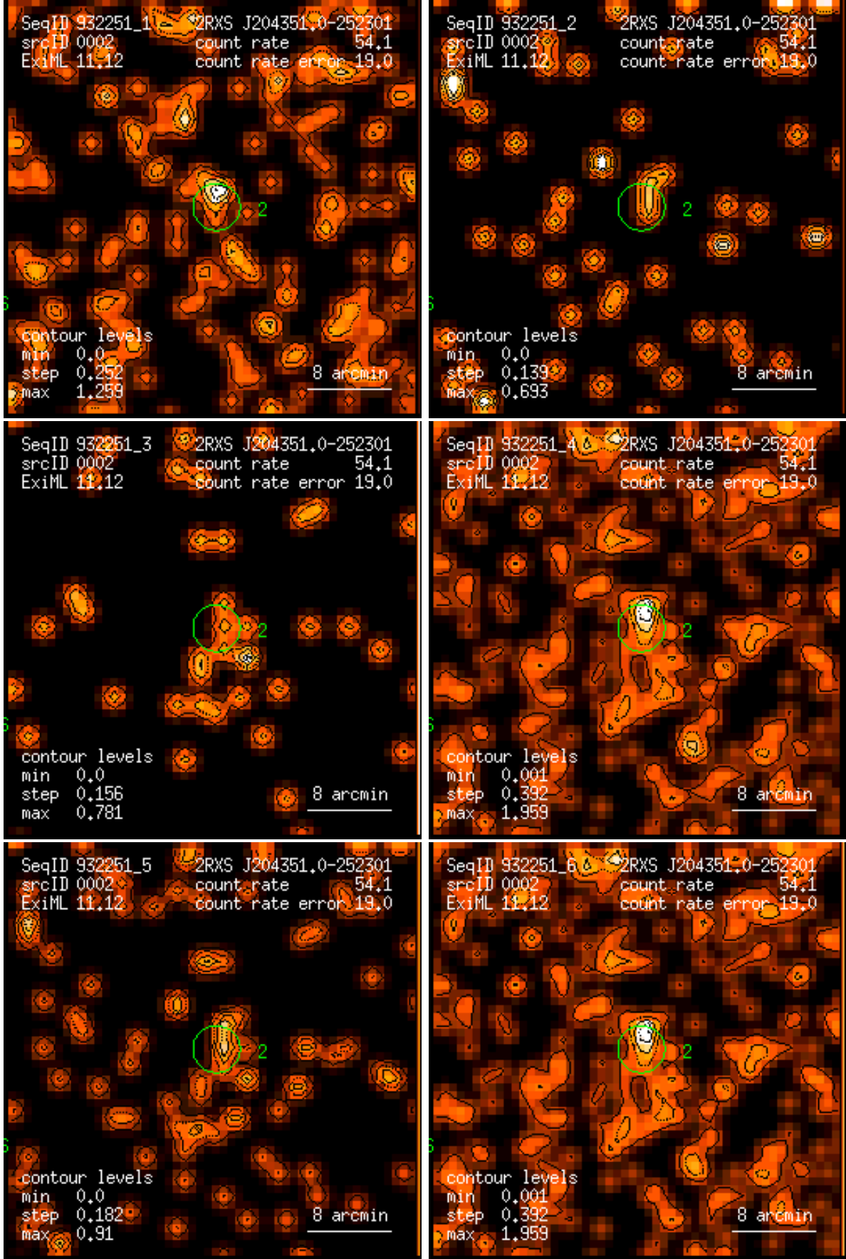
Figure 2: RASS 932251: detection 0002: band rate images, Gaussian filter: (1) PSPC channels 11 – 41, (2) 52 – 90, (3) 91 – 201, (4) 11 – 235, (5) 52 – 201, (6) 11 – 201. Broad band rates in counts/ks. Band rate contour levels in counts/ks/arcmin 2 .
