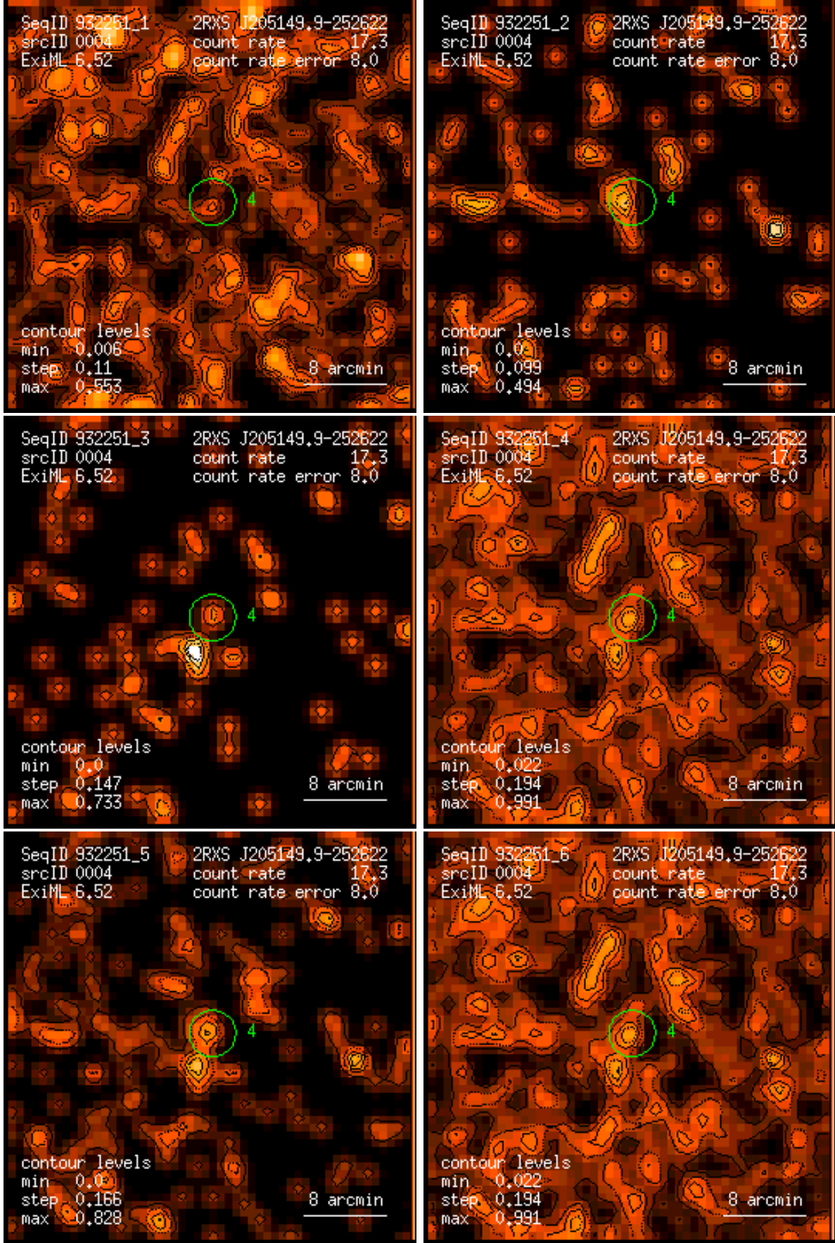
Figure 4: RASS 932251: detection 0004: band rate images, Gaussian filter: (1) PSPC channels 11 – 41, (2) 52 – 90, (3) 91 – 201, (4) 11 – 235, (5) 52 – 201, (6) 11 – 201. Broad band rates in counts/ks. Band rate contour levels in counts/ks/arcmin 2 .
