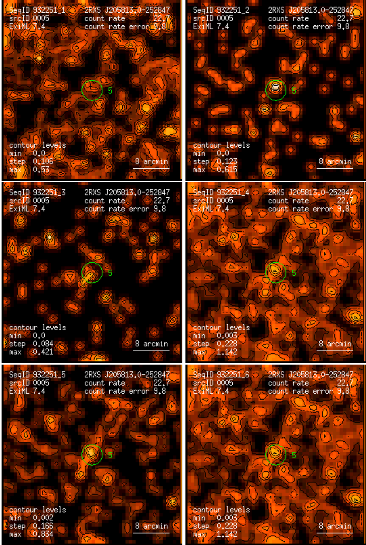
Figure 5: RASS 932251: detection 0005: band rate images, Gaussian filter: (1) PSPC channels 11 – 41, (2) 52 – 90, (3) 91 – 201, (4) 11 – 235, (5) 52 – 201, (6) 11 – 201. Broad band rates in counts/ks. Band rate contour levels in counts/ks/arcmin 2 .
