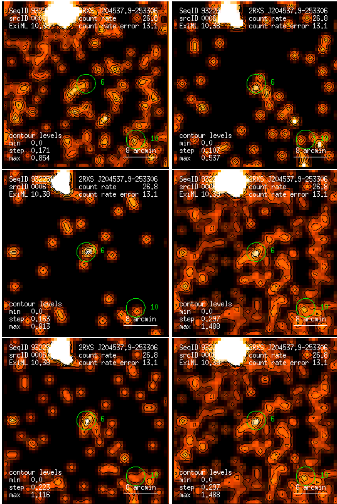
Figure 6: RASS 932251: detection 0006: band rate images, Gaussian filter: (1) PSPC channels 11 – 41, (2) 52 – 90, (3) 91 – 201, (4) 11 – 235, (5) 52 – 201, (6) 11 – 201. Broad band rates in counts/ks. Band rate contour levels in counts/ks/arcmin 2 .
