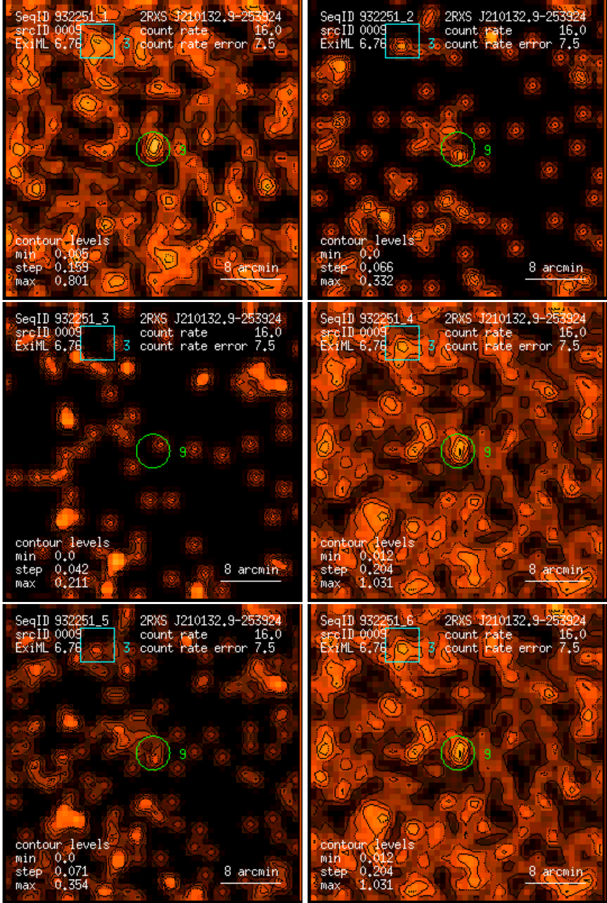
Figure 9: RASS 932251: detection 0009: band rate images, Gaussian filter: (1) PSPC channels 11 – 41, (2) 52 – 90, (3) 91 – 201, (4) 11 – 235, (5) 52 – 201, (6) 11 – 201. Broad band rates in counts/ks. Band rate contour levels in counts/ks/arcmin 2 .
