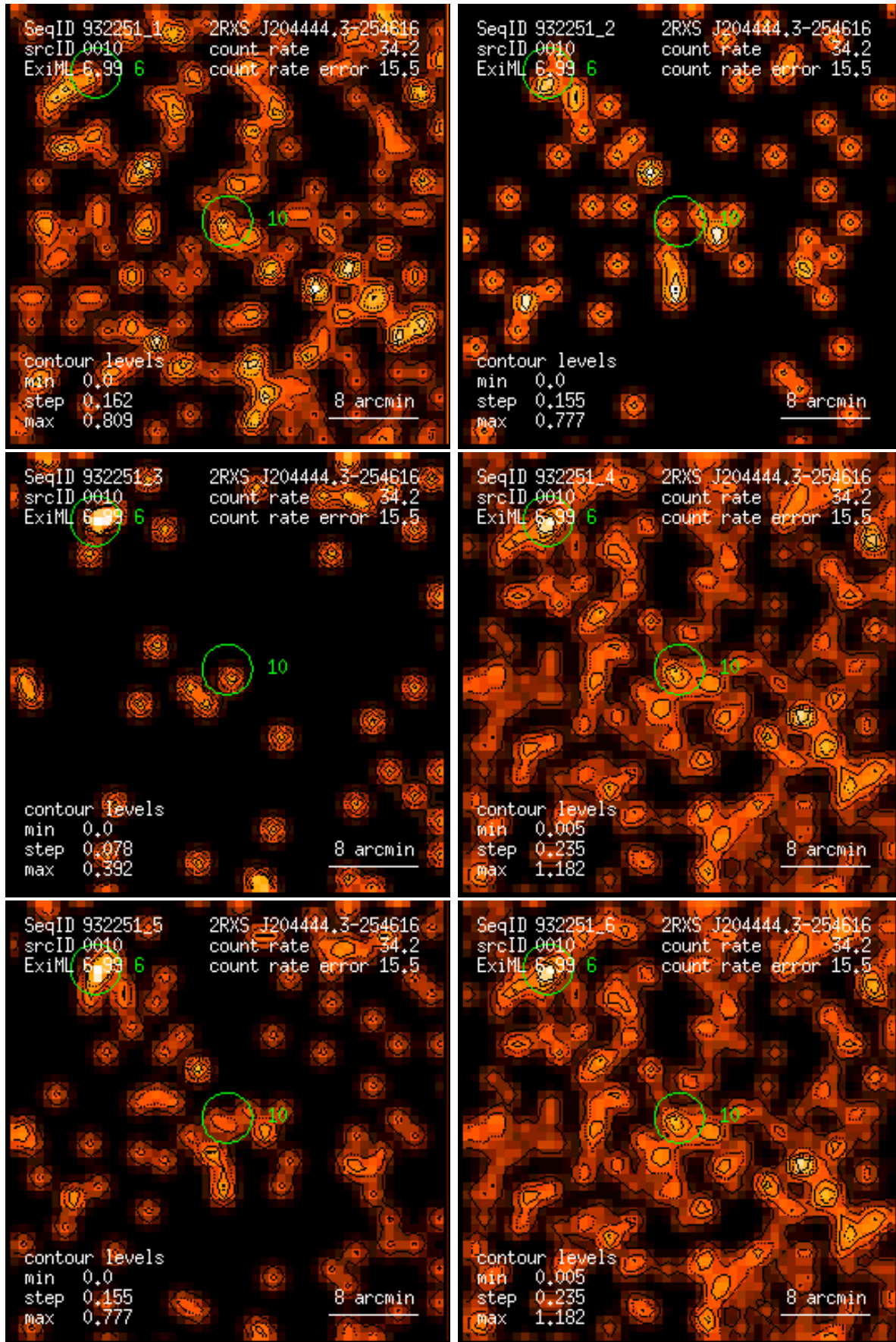
Figure 10: RASS 932251: detection 0010: band rate images, Gaussian filter: (1) PSPC channels 11 – 41, (2) 52 – 90, (3) 91 – 201, (4) 11 – 235, (5) 52 – 201, (6) 11 – 201. Broad band rates in counts/ks. Band rate contour levels in counts/ks/arcmin 2 .
