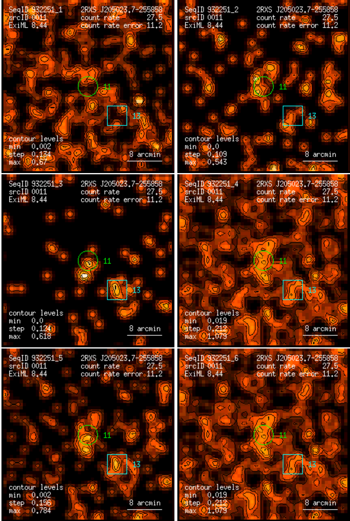
Figure 11: RASS 932251: detection 0011: band rate images, Gaussian filter: (1) PSPC channels 11 – 41, (2) 52 – 90, (3) 91 – 201, (4) 11 – 235, (5) 52 – 201, (6) 11 – 201. Broad band rates in counts/ks. Band rate contour levels in counts/ks/arcmin 2 .
