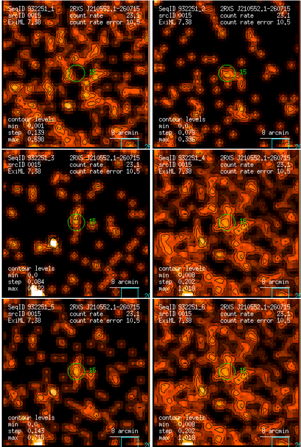
Figure 15: RASS 932251: detection 0015: band rate images, Gaussian filter: (1) PSPC channels 11 – 41, (2) 52 – 90, (3) 91 – 201, (4) 11 – 235, (5) 52 – 201, (6) 11 – 201. Broad band rates in counts/ks. Band rate contour levels in counts/ks/arcmin 2 .
