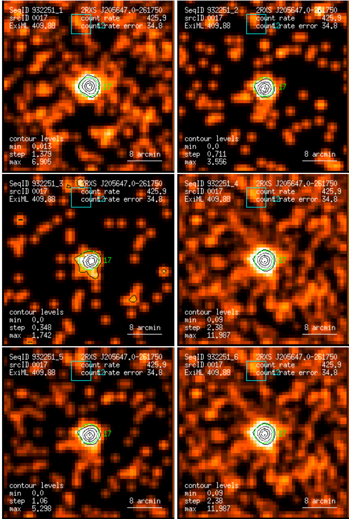
Figure 17: RASS 932251: detection 0017: band rate images, Gaussian filter: (1) PSPC channels 11 – 41, (2) 52 – 90, (3) 91 – 201, (4) 11 – 235, (5) 52 – 201, (6) 11 – 201. Broad band rates in counts/ks. Band rate contour levels in counts/ks/arcmin 2 .
