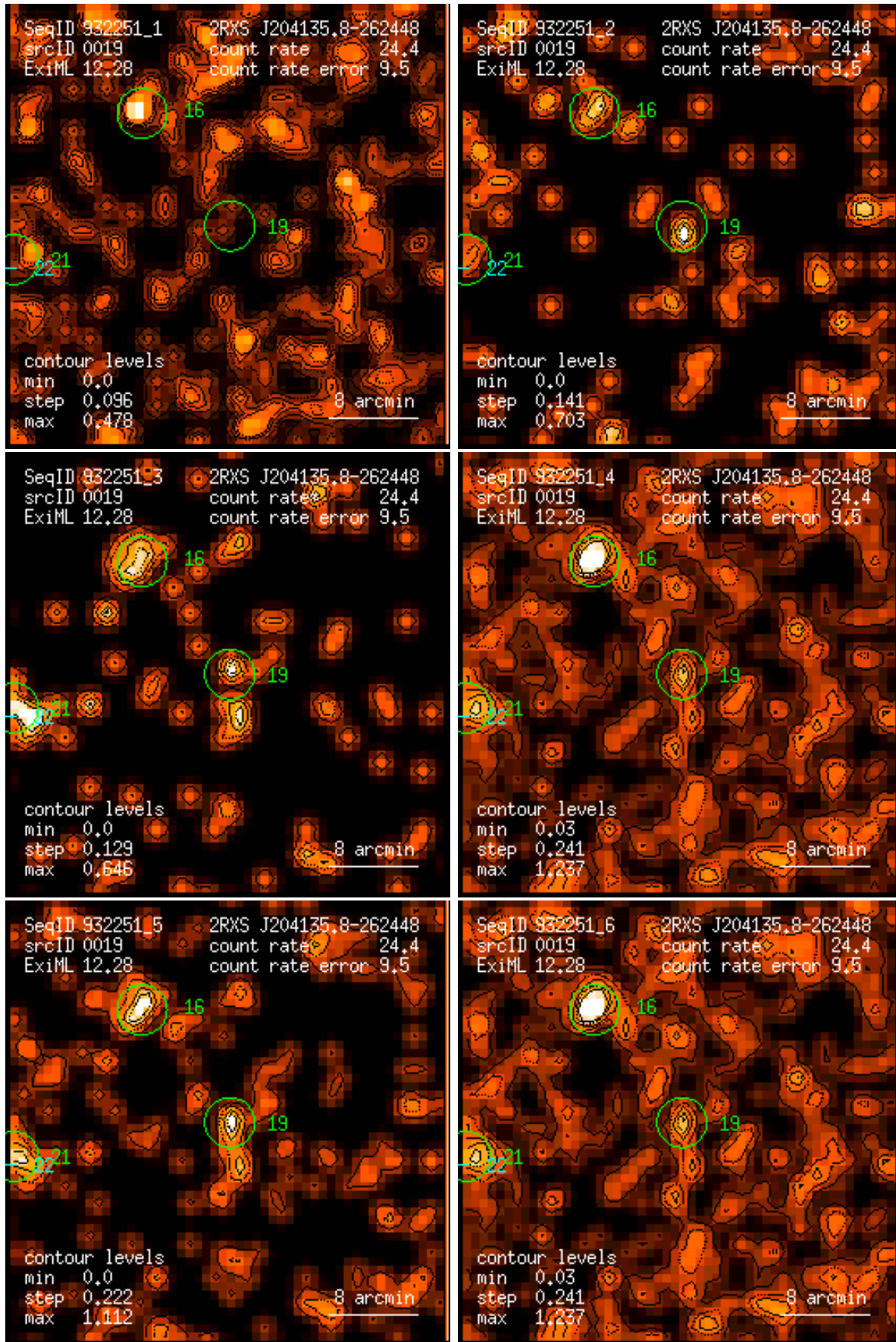
Figure 19: RASS 932251: detection 0019: band rate images, Gaussian filter: (1) PSPC channels 11 – 41, (2) 52 – 90, (3) 91 – 201, (4) 11 – 235, (5) 52 – 201, (6) 11 – 201. Broad band rates in counts/ks. Band rate contour levels in counts/ks/arcmin 2 .
