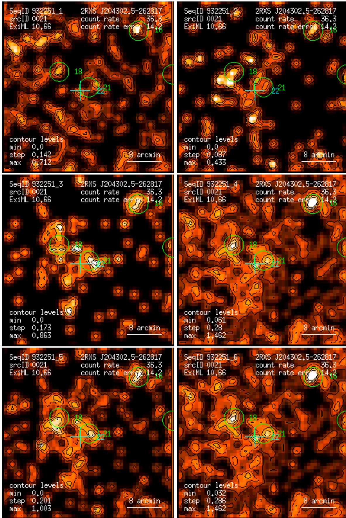
Figure 21: RASS 932251: detection 0021: band rate images, Gaussian filter: (1) PSPC channels 11 – 41, (2) 52 – 90, (3) 91 – 201, (4) 11 – 235, (5) 52 – 201, (6) 11 – 201. Broad band rates in counts/ks. Band rate contour levels in counts/ks/arcmin 2 .
