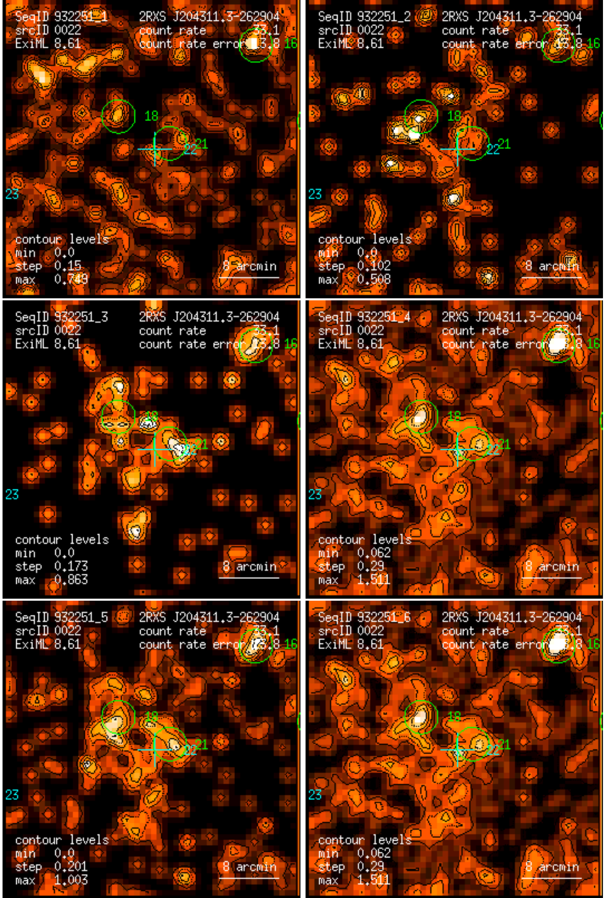
Figure 22: RASS 932251: detection 0022: band rate images, Gaussian filter: (1) PSPC channels 11 – 41, (2) 52 – 90, (3) 91 – 201, (4) 11 – 235, (5) 52 – 201, (6) 11 – 201. Broad band rates in counts/ks. Band rate contour levels in counts/ks/arcmin 2 .
