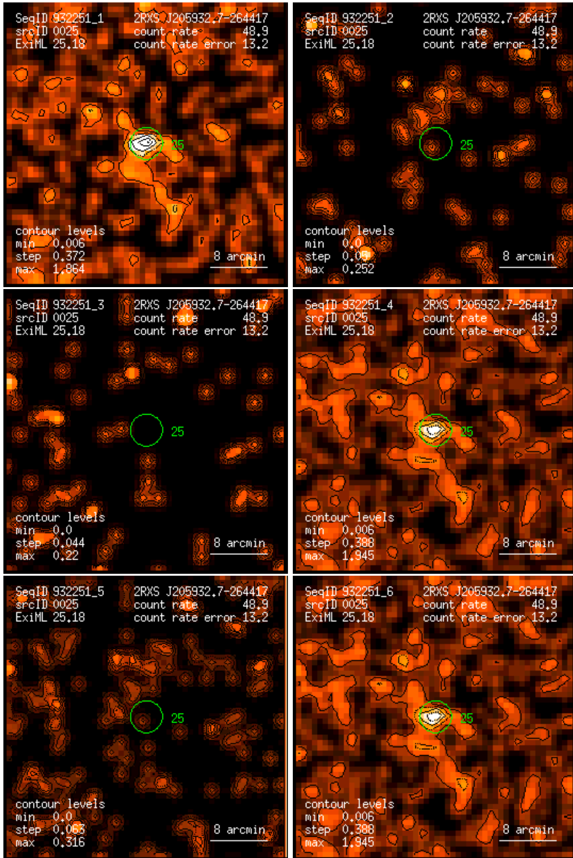
Figure 25: RASS 932251: detection 0025: band rate images, Gaussian filter: (1) PSPC channels 11 – 41, (2) 52 – 90, (3) 91 – 201, (4) 11 – 235, (5) 52 – 201, (6) 11 – 201. Broad band rates in counts/ks. Band rate contour levels in counts/ks/arcmin 2 .
