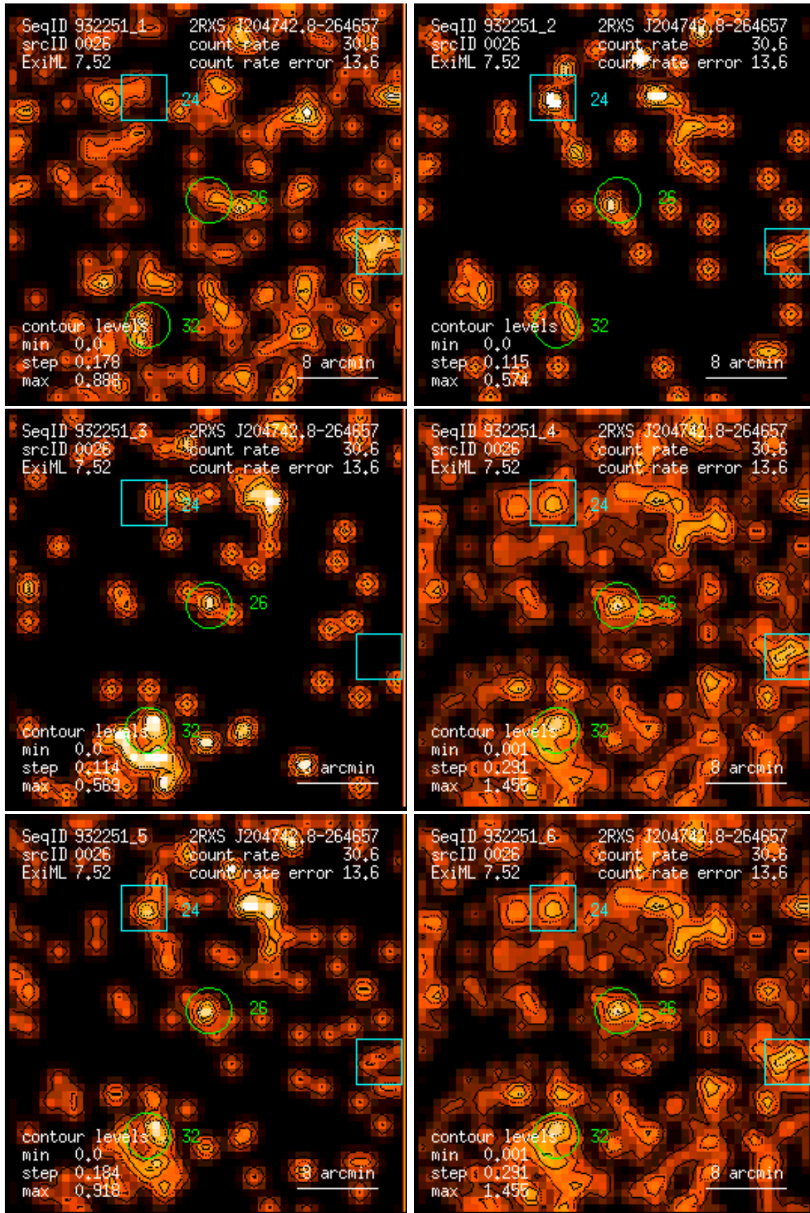
Figure 26: RASS 932251: detection 0026: band rate images, Gaussian filter: (1) PSPC channels 11 – 41, (2) 52 – 90, (3) 91 – 201, (4) 11 – 235, (5) 52 – 201, (6) 11 – 201. Broad band rates in counts/ks. Band rate contour levels in counts/ks/arcmin 2 .
