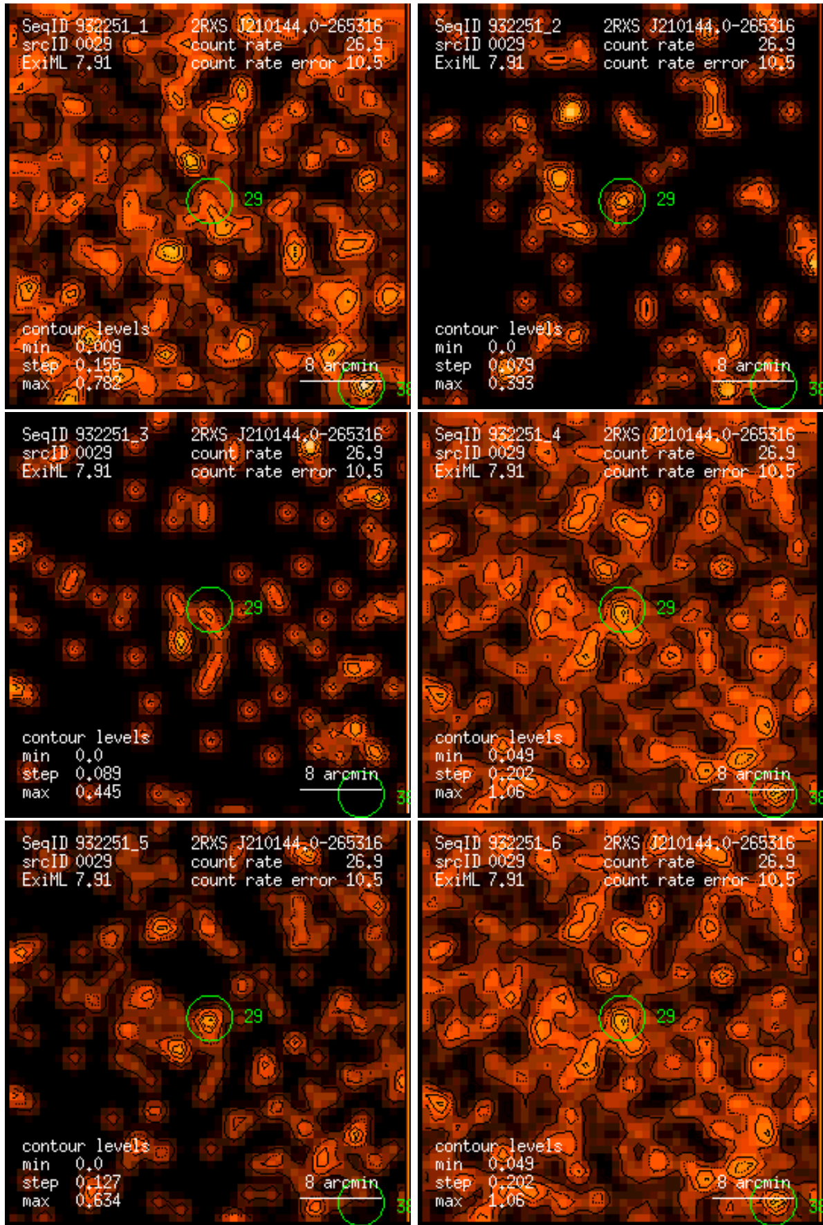
Figure 29: RASS 932251: detection 0029: band rate images, Gaussian filter: (1) PSPC channels 11 – 41, (2) 52 – 90, (3) 91 – 201, (4) 11 – 235, (5) 52 – 201, (6) 11 – 201. Broad band rates in counts/ks. Band rate contour levels in counts/ks/arcmin 2 .
