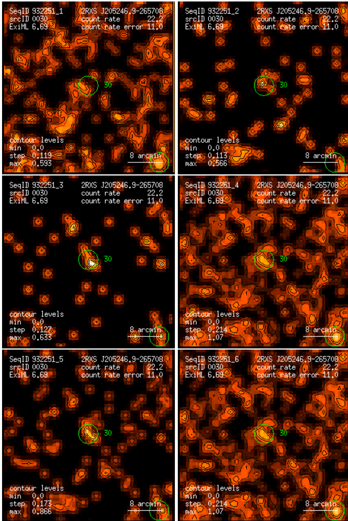
Figure 30: RASS 932251: detection 0030: band rate images, Gaussian filter: (1) PSPC channels 11 – 41, (2) 52 – 90, (3) 91 – 201, (4) 11 – 235, (5) 52 – 201, (6) 11 – 201. Broad band rates in counts/ks. Band rate contour levels in counts/ks/arcmin 2 .
