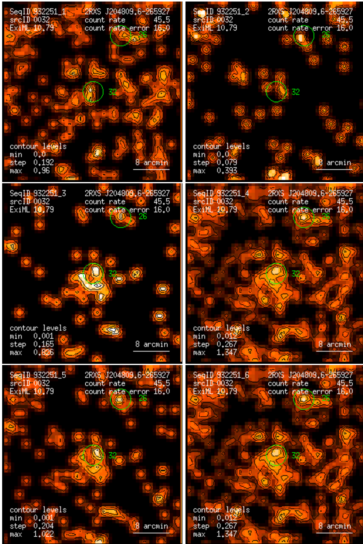
Figure 32: RASS 932251: detection 0032: band rate images, Gaussian filter: (1) PSPC channels 11 – 41, (2) 52 – 90, (3) 91 – 201, (4) 11 – 235, (5) 52 – 201, (6) 11 – 201. Broad band rates in counts/ks. Band rate contour levels in counts/ks/arcmin 2 .
