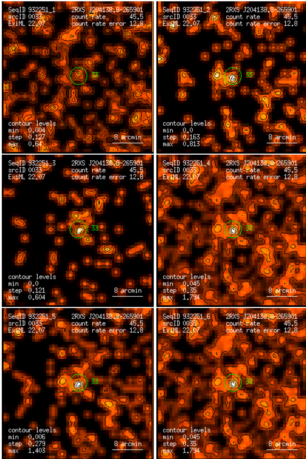
Figure 33: RASS 932251: detection 0033: band rate images, Gaussian filter: (1) PSPC channels 11 – 41, (2) 52 – 90, (3) 91 – 201, (4) 11 – 235, (5) 52 – 201, (6) 11 – 201. Broad band rates in counts/ks. Band rate contour levels in counts/ks/arcmin 2 .
