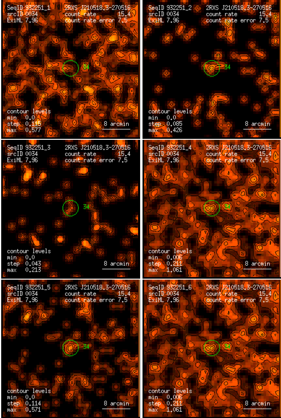
Figure 34: RASS 932251: detection 0034: band rate images, Gaussian filter: (1) PSPC channels 11 – 41, (2) 52 – 90, (3) 91 – 201, (4) 11 – 235, (5) 52 – 201, (6) 11 – 201. Broad band rates in counts/ks. Band rate contour levels in counts/ks/arcmin 2 .
