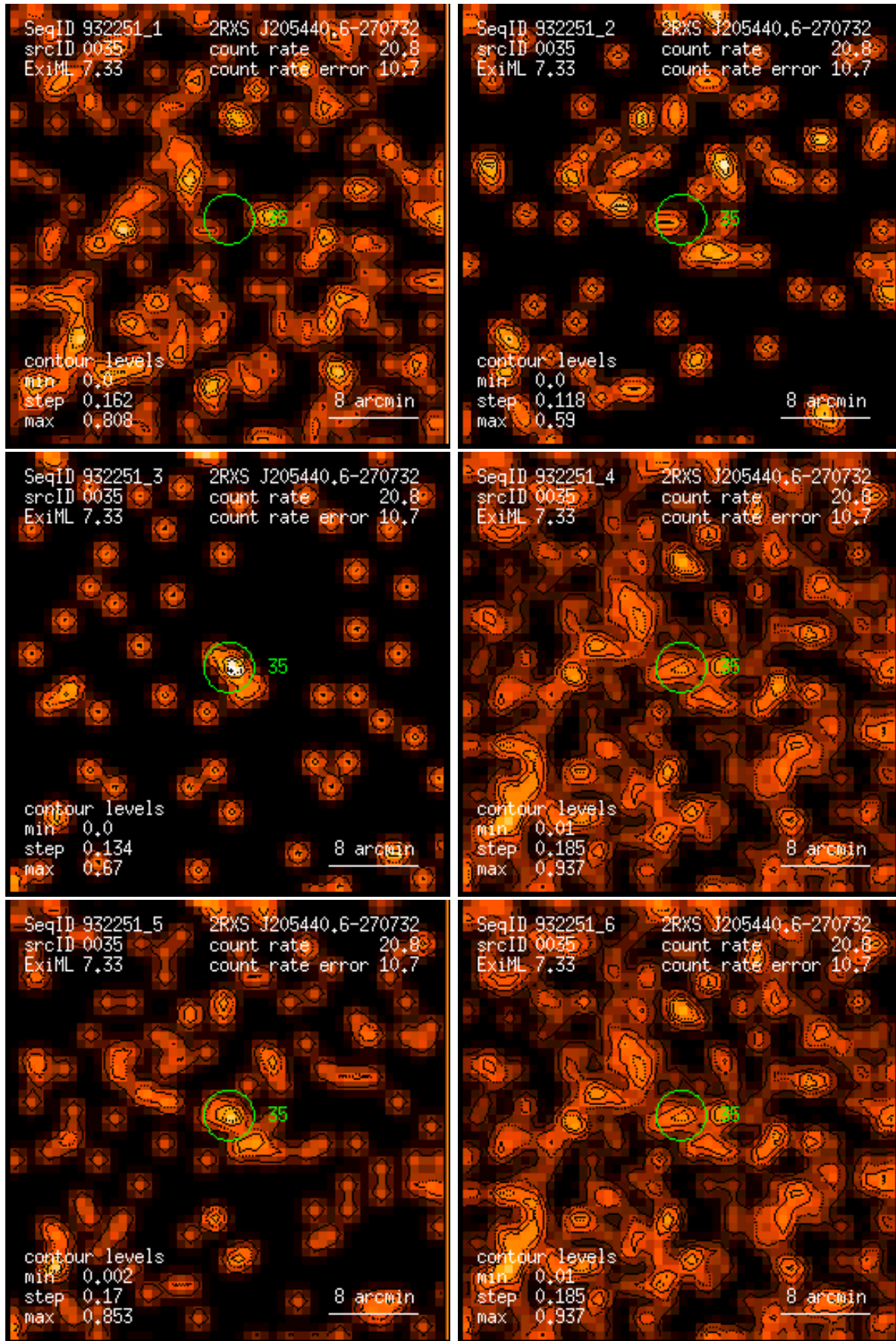
Figure 35: RASS 932251: detection 0035: band rate images, Gaussian filter: (1) PSPC channels 11 – 41, (2) 52 – 90, (3) 91 – 201, (4) 11 – 235, (5) 52 – 201, (6) 11 – 201. Broad band rates in counts/ks. Band rate contour levels in counts/ks/arcmin 2 .
