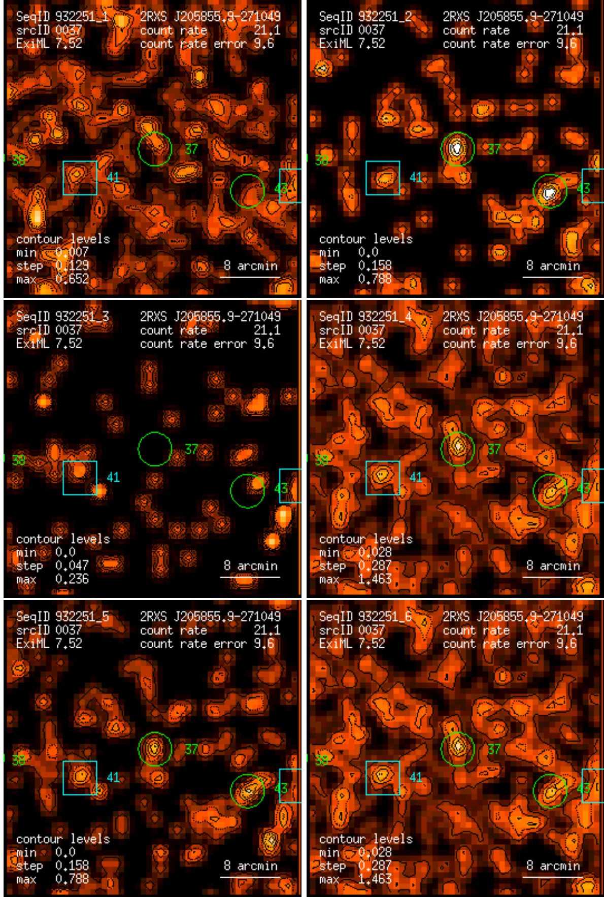
Figure 37: RASS 932251: detection 0037: band rate images, Gaussian filter: (1) PSPC channels 11 – 41, (2) 52 – 90, (3) 91 – 201, (4) 11 – 235, (5) 52 – 201, (6) 11 – 201. Broad band rates in counts/ks. Band rate contour levels in counts/ks/arcmin 2 .
