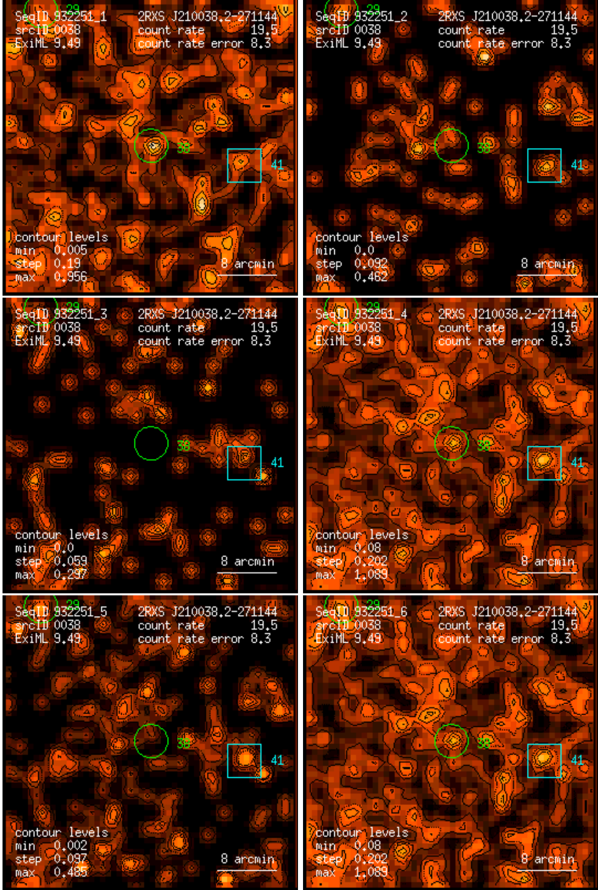
Figure 38: RASS 932251: detection 0038: band rate images, Gaussian filter: (1) PSPC channels 11 – 41, (2) 52 – 90, (3) 91 – 201, (4) 11 – 235, (5) 52 – 201, (6) 11 – 201. Broad band rates in counts/ks. Band rate contour levels in counts/ks/arcmin 2 .
