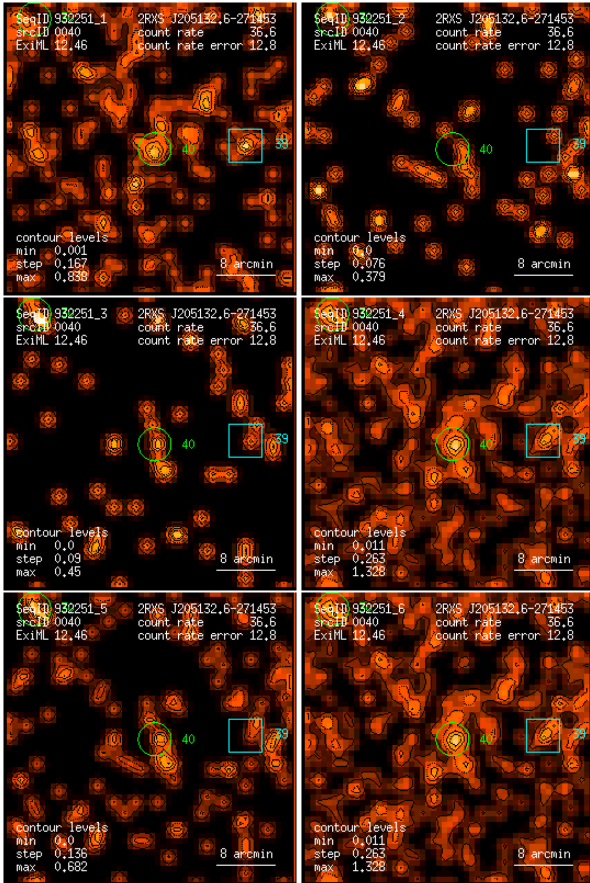
Figure 40: RASS 932251: detection 0040: band rate images, Gaussian filter: (1) PSPC channels 11 – 41, (2) 52 – 90, (3) 91 – 201, (4) 11 – 235, (5) 52 – 201, (6) 11 – 201. Broad band rates in counts/ks. Band rate contour levels in counts/ks/arcmin 2 .
