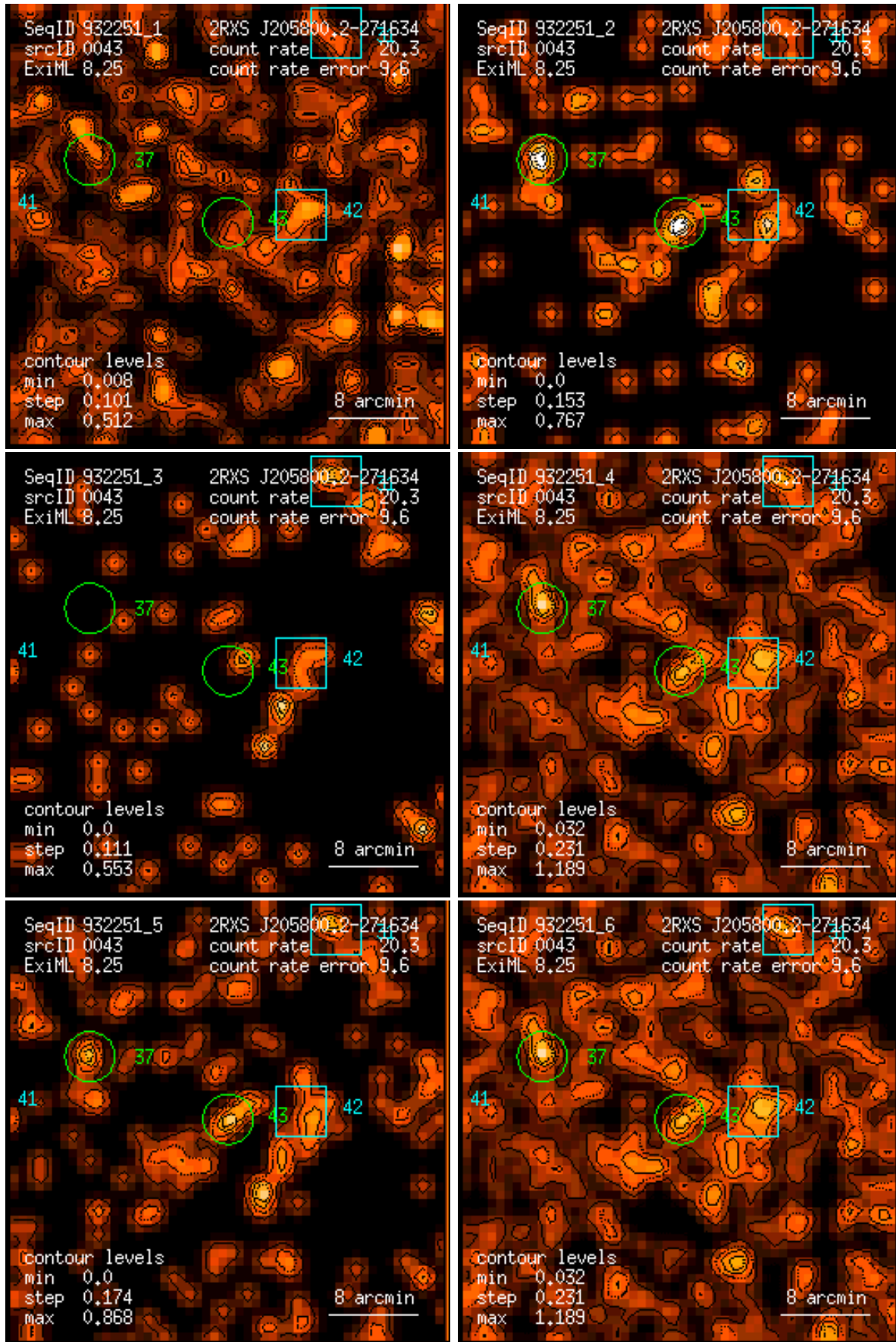
Figure 43: RASS 932251: detection 0043: band rate images, Gaussian filter: (1) PSPC channels 11 – 41, (2) 52 – 90, (3) 91 – 201, (4) 11 – 235, (5) 52 – 201, (6) 11 – 201. Broad band rates in counts/ks. Band rate contour levels in counts/ks/arcmin 2 .
