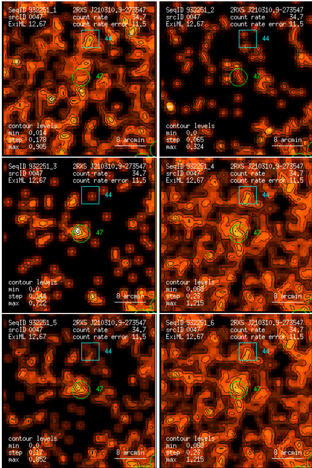
Figure 47: RASS 932251: detection 0047: band rate images, Gaussian filter: (1) PSPC channels 11 – 41, (2) 52 – 90, (3) 91 – 201, (4) 11 – 235, (5) 52 – 201, (6) 11 – 201. Broad band rates in counts/ks. Band rate contour levels in counts/ks/arcmin 2 .
