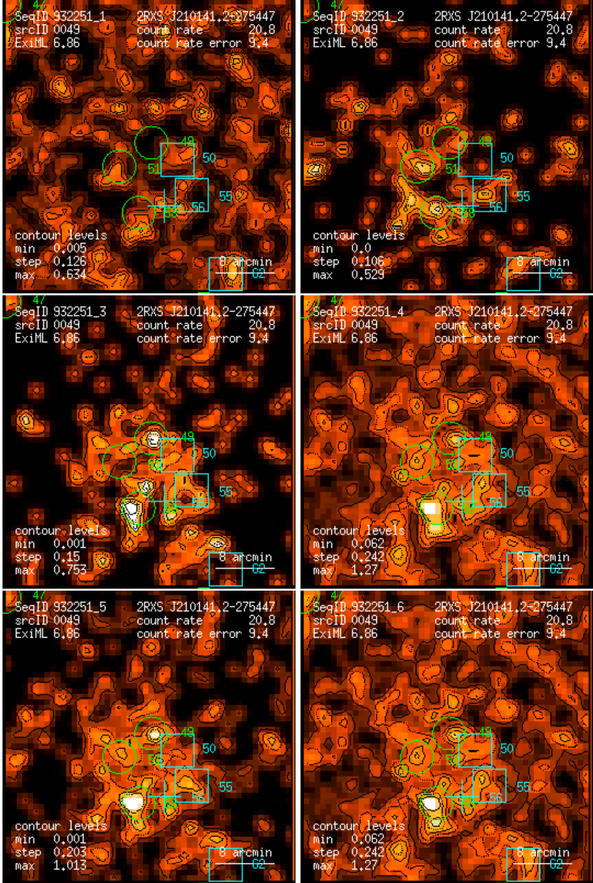
Figure 49: RASS 932251: detection 0049: band rate images, Gaussian filter: (1) PSPC channels 11 – 41, (2) 52 – 90, (3) 91 – 201, (4) 11 – 235, (5) 52 – 201, (6) 11 – 201. Broad band rates in counts/ks. Band rate contour levels in counts/ks/arcmin 2 .
