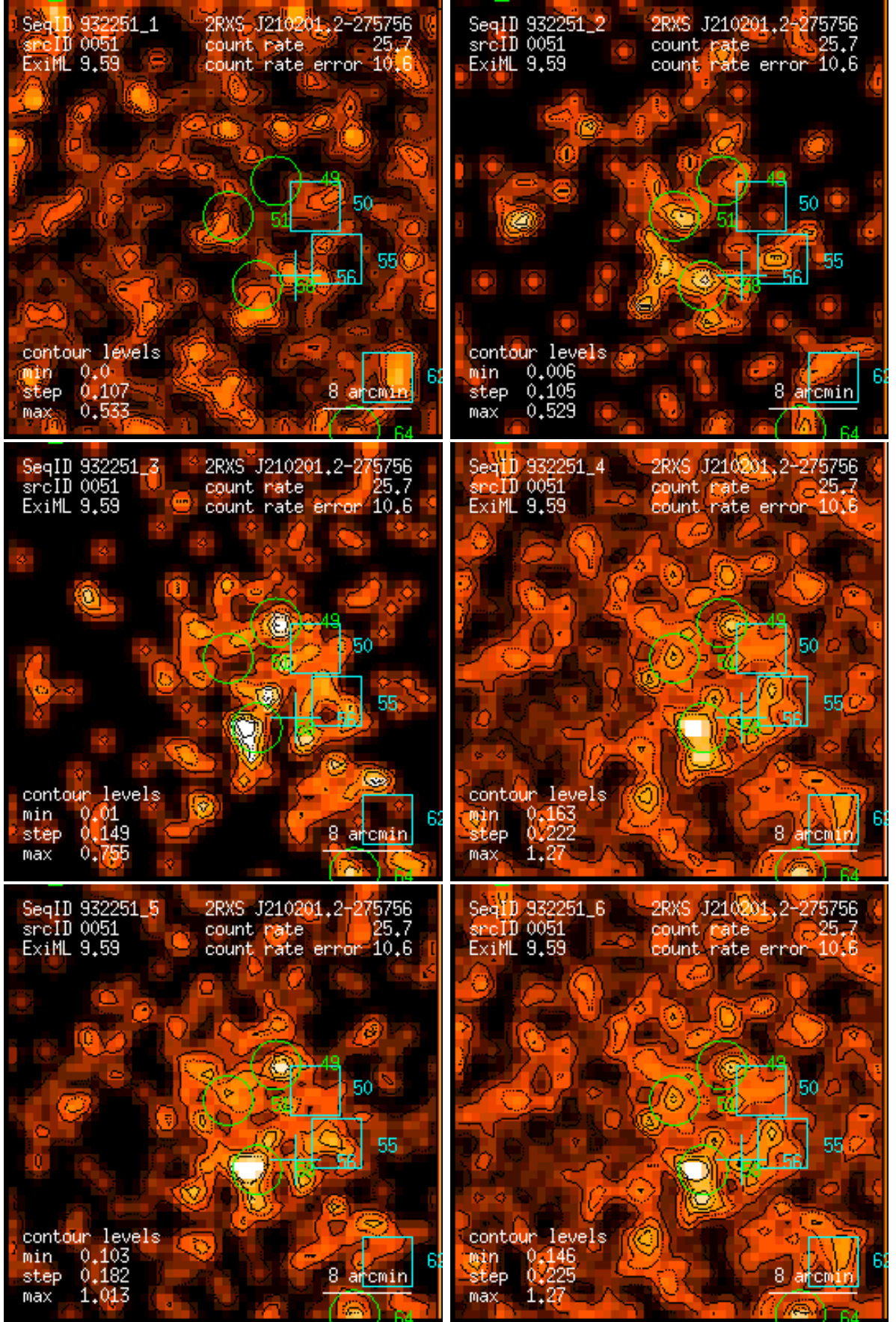
Figure 51: RASS 932251: detection 0051: band rate images, Gaussian filter: (1) PSPC channels 11 – 41, (2) 52 – 90, (3) 91 – 201, (4) 11 – 235, (5) 52 – 201, (6) 11 – 201. Broad band rates in counts/ks. Band rate contour levels in counts/ks/arcmin 2 .
