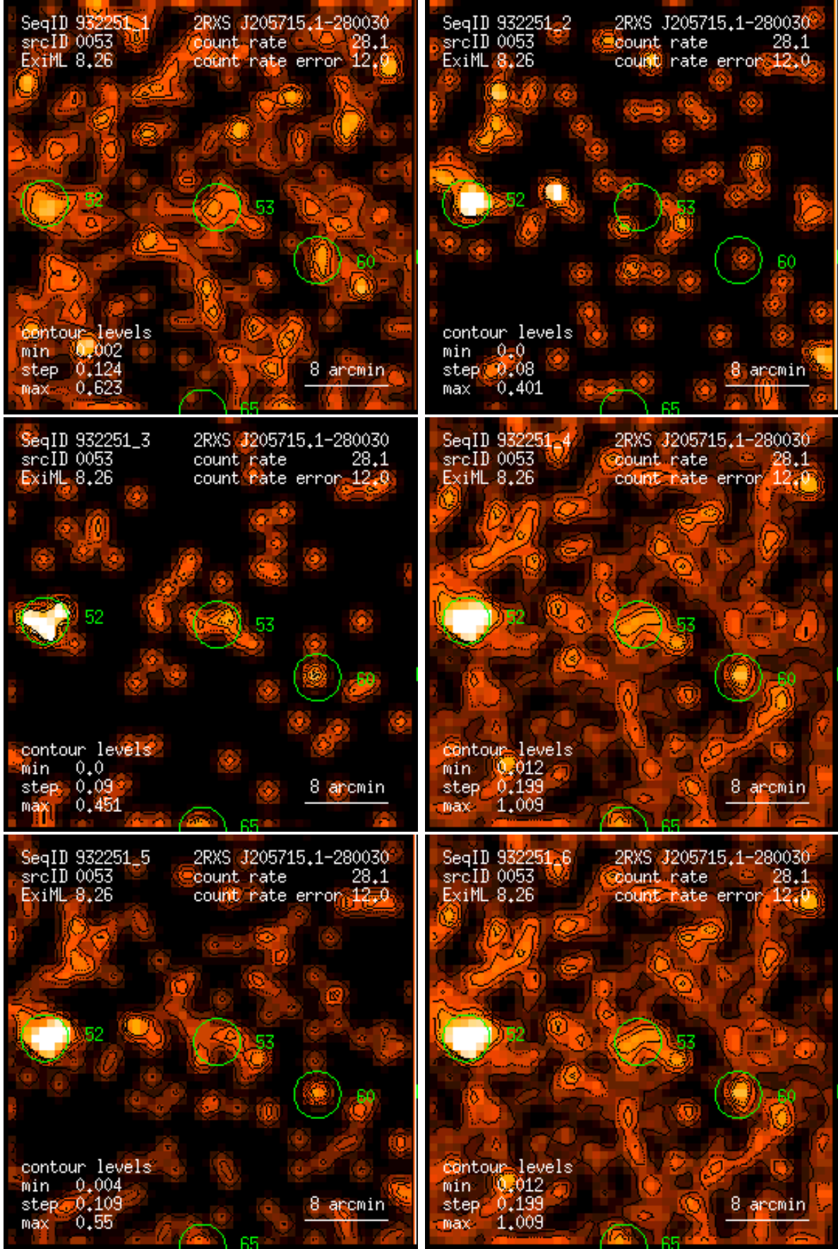
Figure 53: RASS 932251: detection 0053: band rate images, Gaussian filter: (1) PSPC channels 11 – 41, (2) 52 – 90, (3) 91 – 201, (4) 11 – 235, (5) 52 – 201, (6) 11 – 201. Broad band rates in counts/ks. Band rate contour levels in counts/ks/arcmin 2 .
