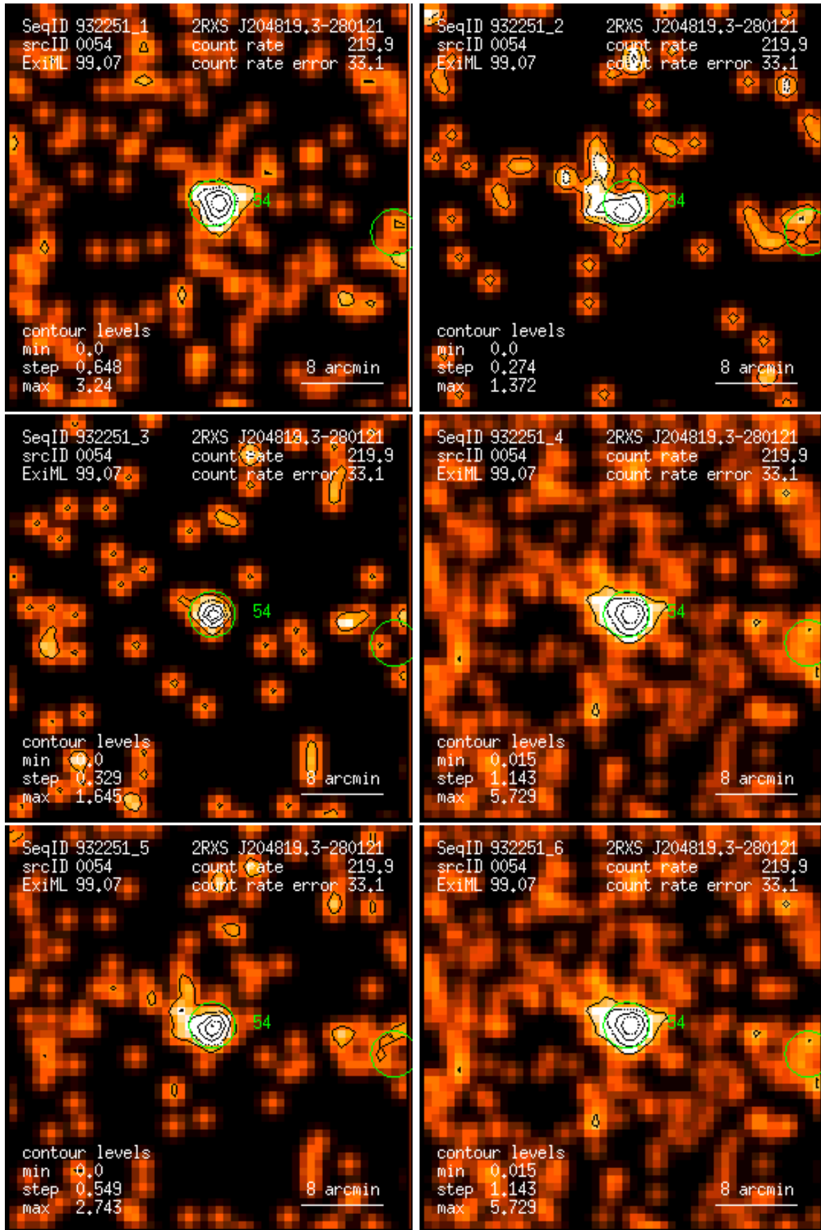
Figure 54: RASS 932251: detection 0054: band rate images, Gaussian filter: (1) PSPC channels 11 – 41, (2) 52 – 90, (3) 91 – 201, (4) 11 – 235, (5) 52 – 201, (6) 11 – 201. Broad band rates in counts/ks. Band rate contour levels in counts/ks/arcmin 2 .
