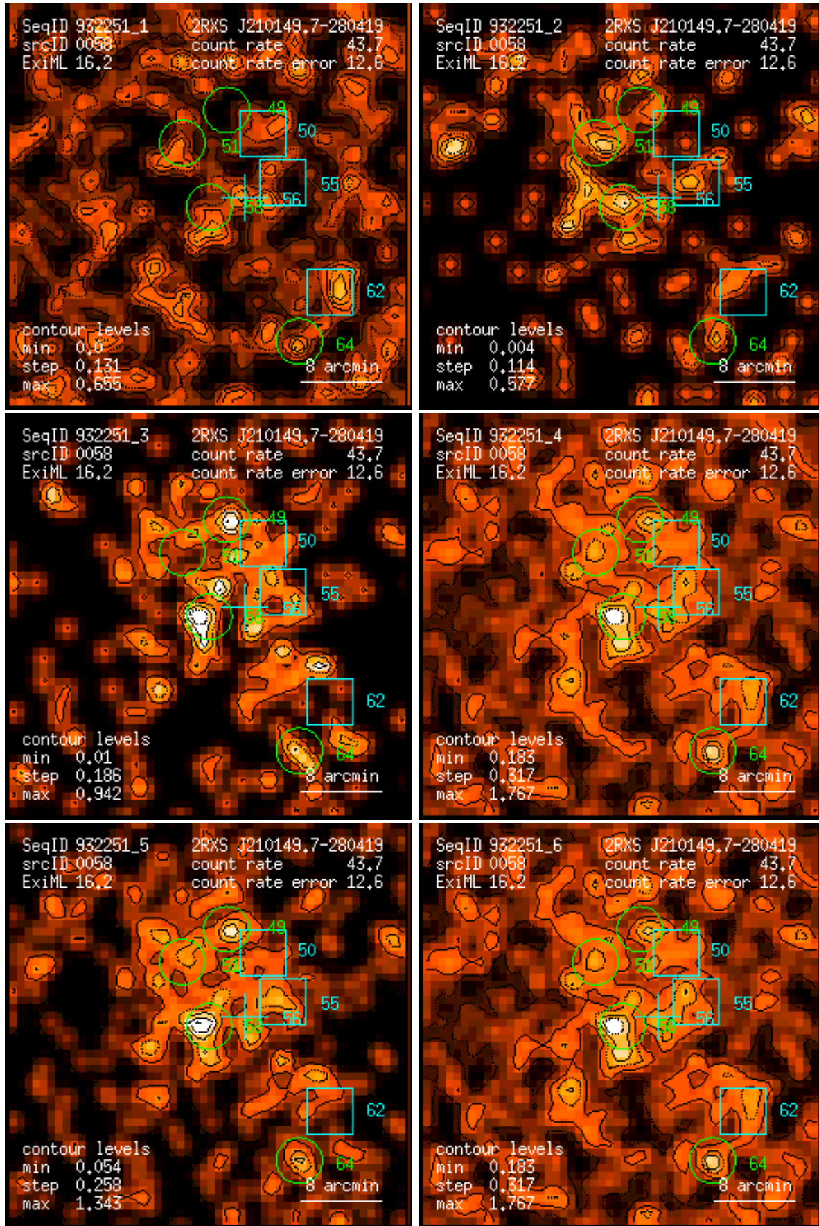
Figure 58: RASS 932251: detection 0058: band rate images, Gaussian filter: (1) PSPC channels 11 – 41, (2) 52 – 90, (3) 91 – 201, (4) 11 – 235, (5) 52 – 201, (6) 11 – 201. Broad band rates in counts/ks. Band rate contour levels in counts/ks/arcmin 2 .
