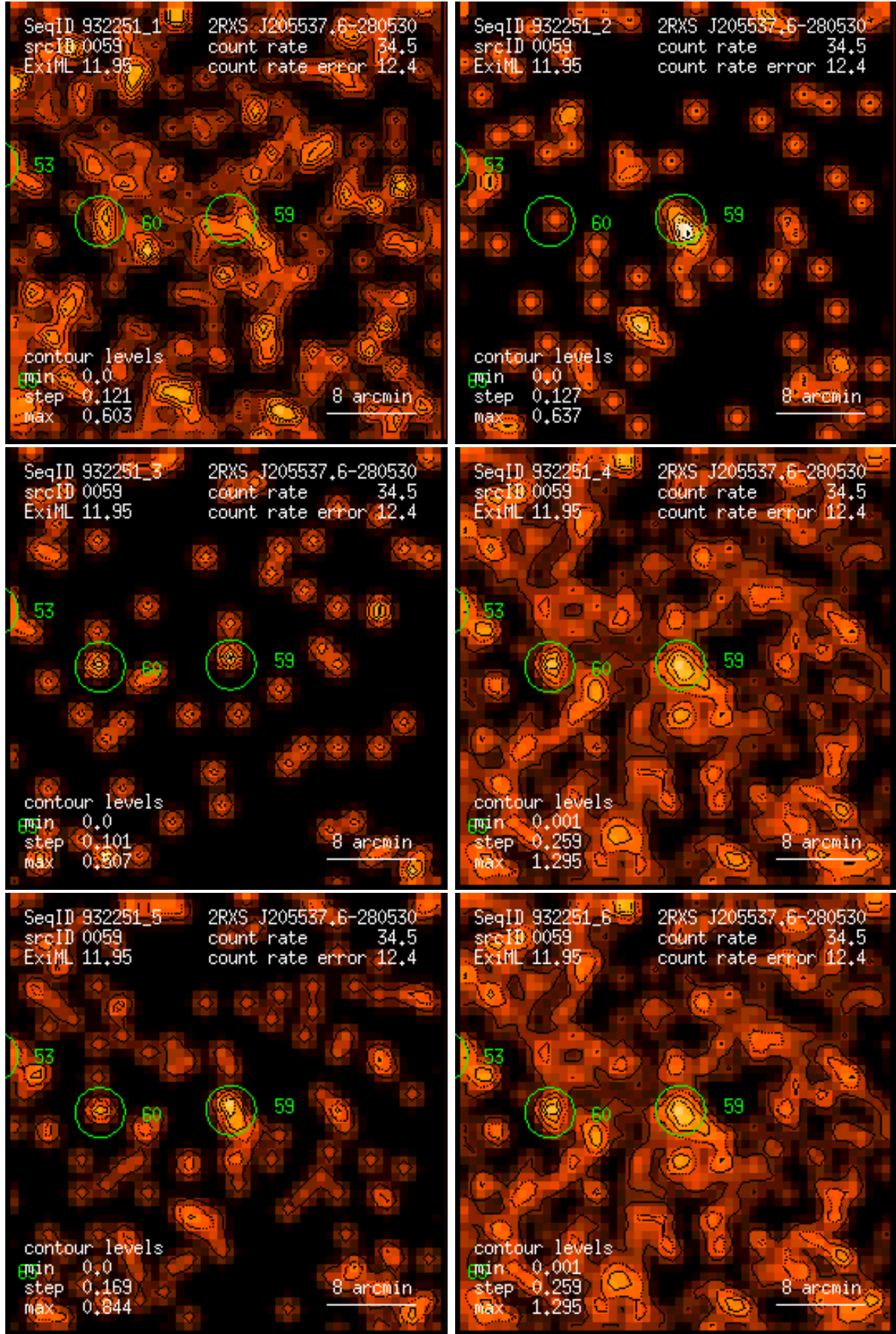
Figure 59: RASS 932251: detection 0059: band rate images, Gaussian filter: (1) PSPC channels 11 – 41, (2) 52 – 90, (3) 91 – 201, (4) 11 – 235, (5) 52 – 201, (6) 11 – 201. Broad band rates in counts/ks. Band rate contour levels in counts/ks/arcmin 2 .
