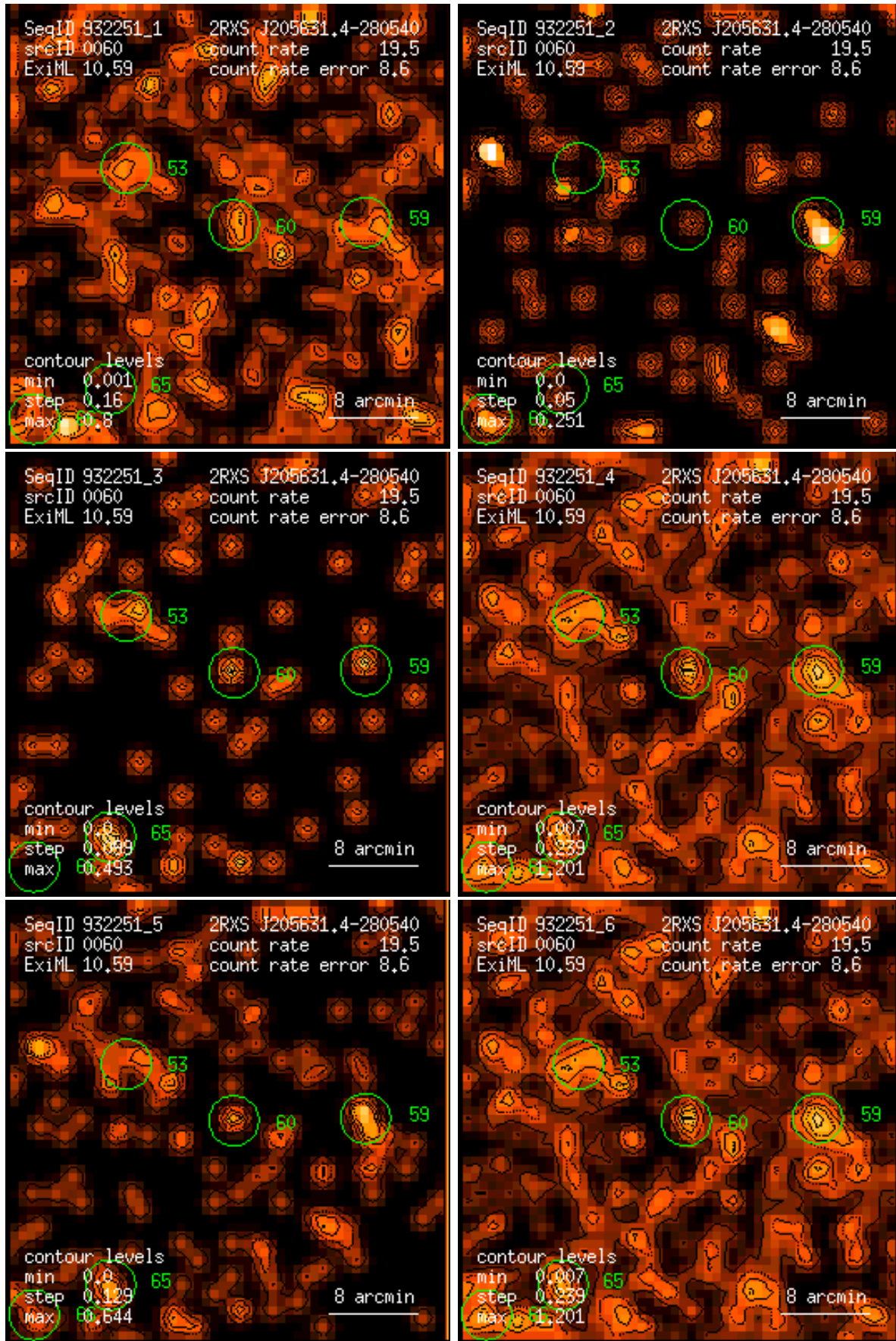
Figure 60: RASS 932251: detection 0060: band rate images, Gaussian filter: (1) PSPC channels 11 – 41, (2) 52 – 90, (3) 91 – 201, (4) 11 – 235, (5) 52 – 201, (6) 11 – 201. Broad band rates in counts/ks. Band rate contour levels in counts/ks/arcmin 2 .
