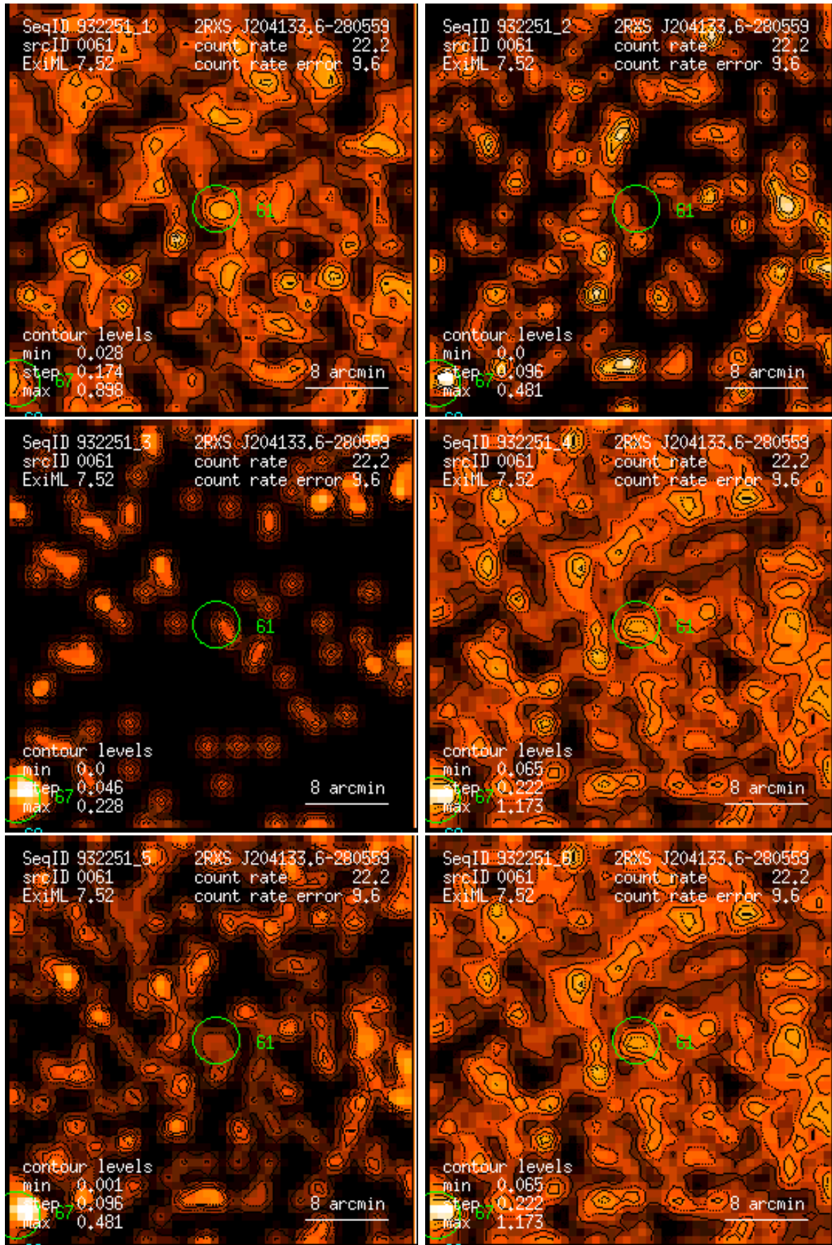
Figure 61: RASS 932251: detection 0061: band rate images, Gaussian filter: (1) PSPC channels 11 – 41, (2) 52 – 90, (3) 91 – 201, (4) 11 – 235, (5) 52 – 201, (6) 11 – 201. Broad band rates in counts/ks. Band rate contour levels in counts/ks/arcmin 2 .
