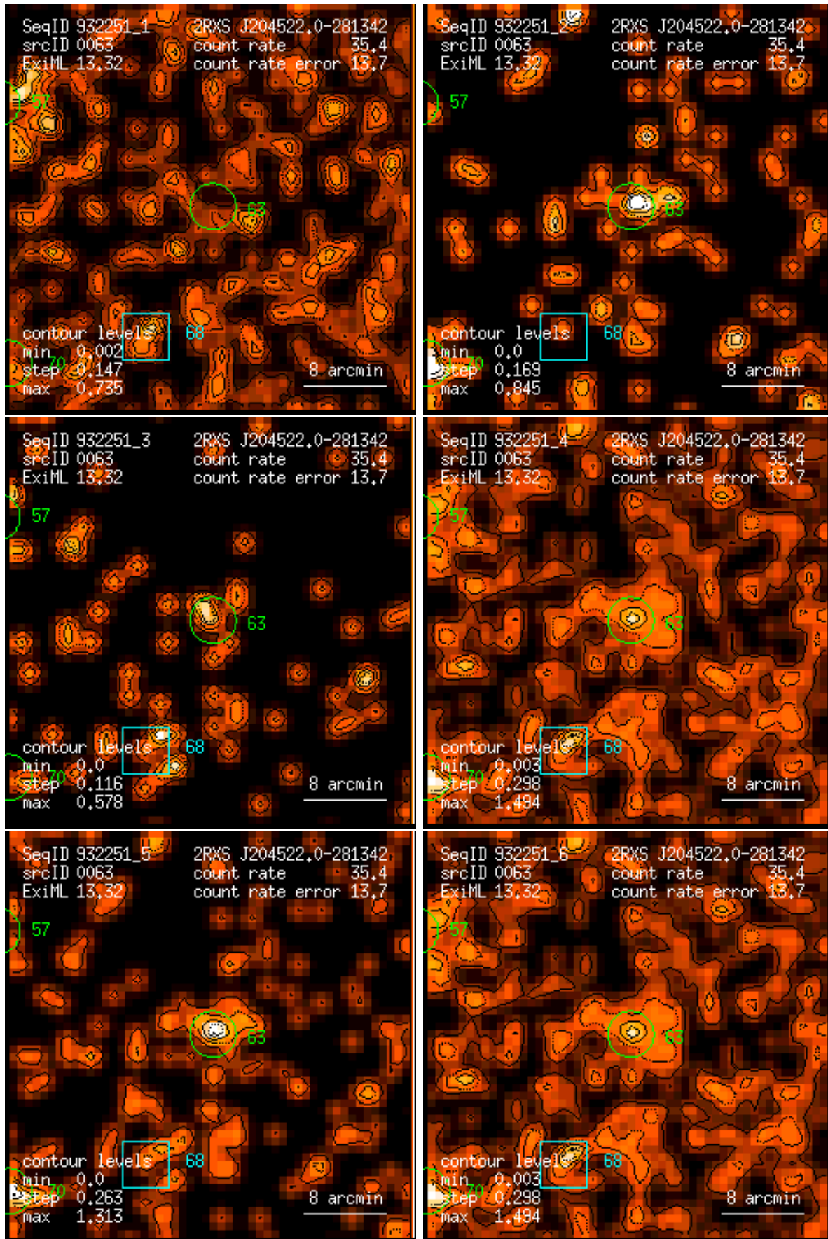
Figure 63: RASS 932251: detection 0063: band rate images, Gaussian filter: (1) PSPC channels 11 – 41, (2) 52 – 90, (3) 91 – 201, (4) 11 – 235, (5) 52 – 201, (6) 11 – 201. Broad band rates in counts/ks. Band rate contour levels in counts/ks/arcmin 2 .
