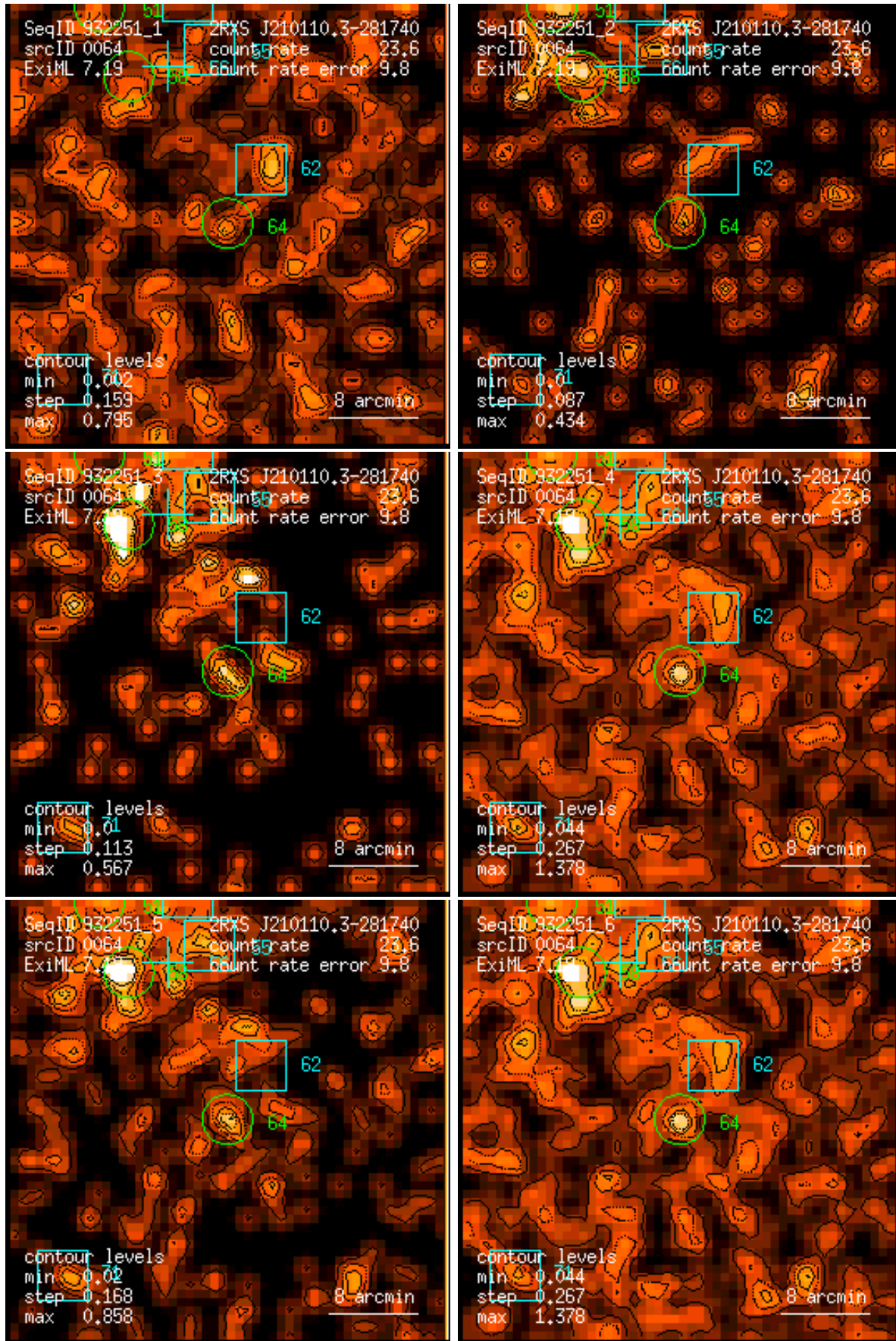
Figure 64: RASS 932251: detection 0064: band rate images, Gaussian filter: (1) PSPC channels 11 – 41, (2) 52 – 90, (3) 91 – 201, (4) 11 – 235, (5) 52 – 201, (6) 11 – 201. Broad band rates in counts/ks. Band rate contour levels in counts/ks/arcmin 2 .
