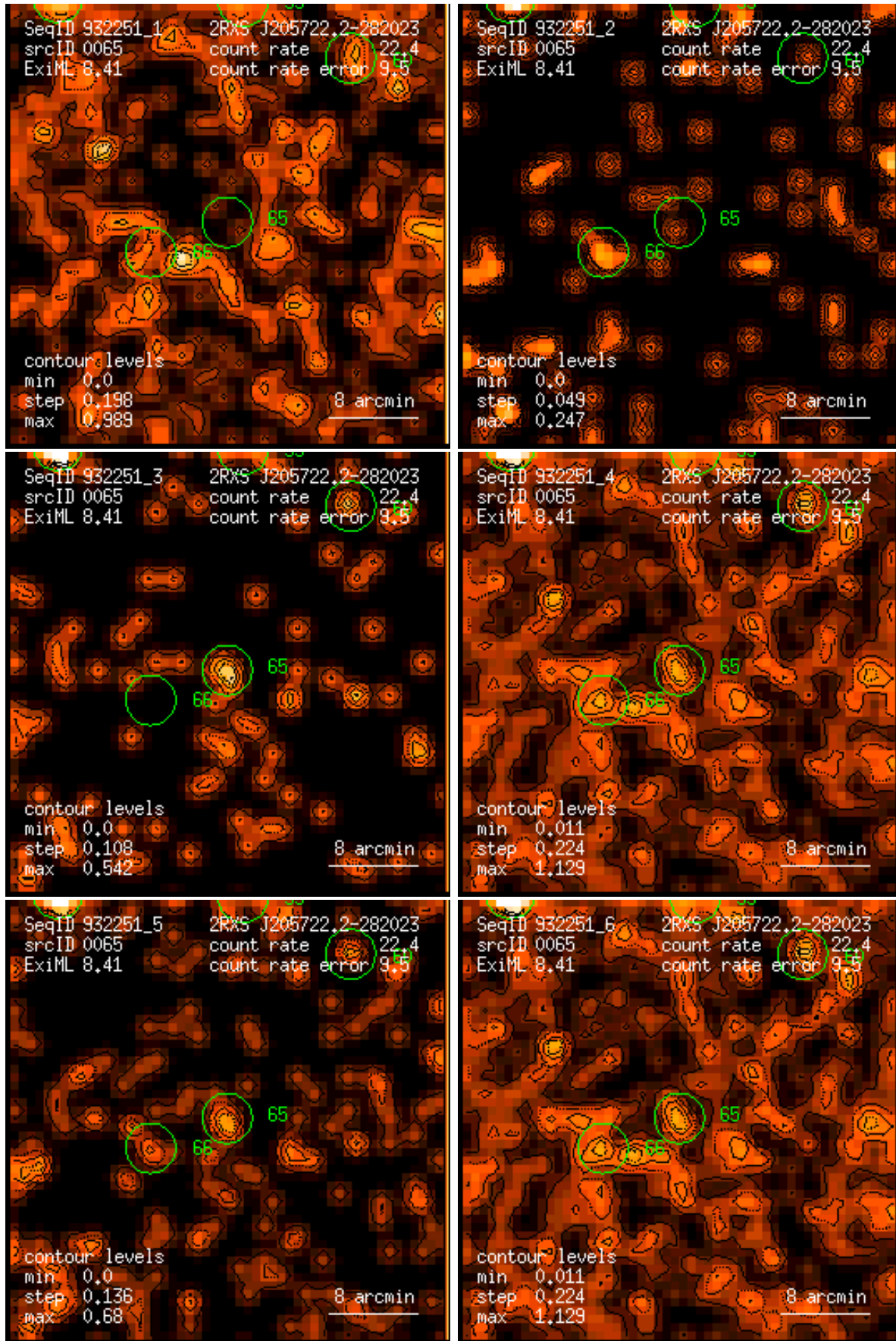
Figure 65: RASS 932251: detection 0065: band rate images, Gaussian filter: (1) PSPC channels 11 – 41, (2) 52 – 90, (3) 91 – 201, (4) 11 – 235, (5) 52 – 201, (6) 11 – 201. Broad band rates in counts/ks. Band rate contour levels in counts/ks/arcmin 2 .
